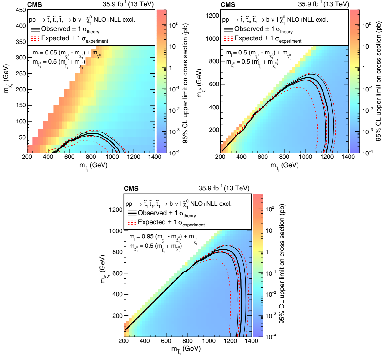
FIG. 12. Expected and observed limits for the T8bb \ell\ell\nu\nu model with \tilde{t}_1 \rightarrow b\tilde{\chi}_1^+ and bv\tilde{\ell} \rightarrow bv\tilde{\ell}\tilde{\chi}_1^0 decays in the m_{\tilde{t}_1} - m_{\tilde{\chi}_1^0} mass plane for three different mass configurations defined by m_{\tilde{\chi}_1^0} = x(m_{\tilde{t}_1} - m_{\tilde{\chi}_1^0}) + m_{\tilde{\chi}_1^0} with x = 0.05 (upper left), x = 0.5 (upper right), and x = 0.95 (lower). The description of curves is the same as in the caption of Fig. 11.
