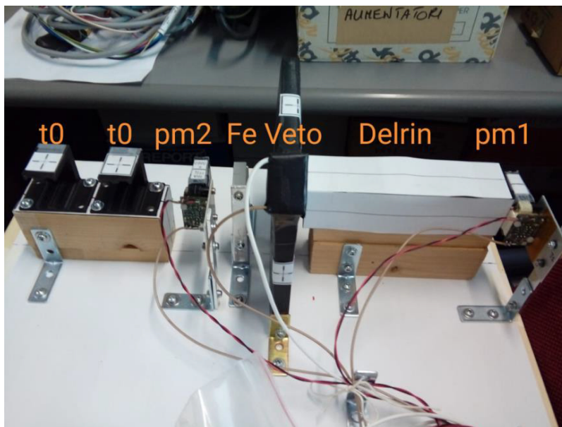
Figure 19. Experimental setup for the selection of charge exchange events with converted photons. “pm1” and “pm2” are the 3×3 cm 2 scintillator pads. VETO is the 15×15 cm 2 pad used to veto charged particles produced after the Delrin block. The trigger is given by the coincidence of pm1 and pm2 and the anti-coincidence of VETO.
