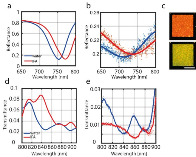
Figure 5. (a) Simulated spectral shift of the reflected light when a thin film of distilled water (blue line) or isopropyl alcohol (red line) covers the NP array with periodicity p = 630 nm. (b) Reflectance spectra measured with the array immersed in distilled water (blue dots) or IPA (red dots). Blue and red lines, serving as a guide to the eye, are obtained by interpolating the data with second-order Fourier series. (c) Dark field images of a NP array with periodicity p = 550 nm covered in air (top) or IPA (bottom). Scale bar is 15 \mu\text{m} . (d) As in (a) for transmitted light for a NPs array with p = 630 nm. (e) Transmittance spectra measured with the array immersed in distilled water (blue dots) or IPA (red dots). Blue and red lines represent a moving average of the spectra over 3 nm.
