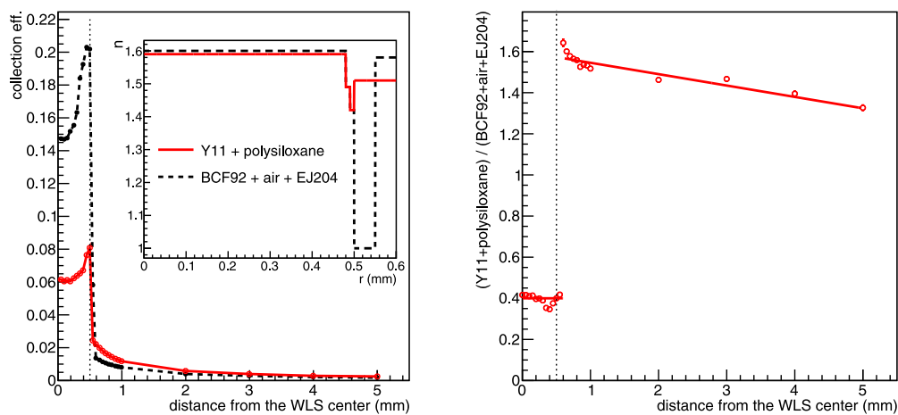
Fig. 2. GEANT4 optical simulation results. Left: Collection efficiency as a function of the distance from the WLS center for the Y11 + polysiloxane (solid red) and the BCF92 + air + EJ204 (dashed black) setups. Right: ratio of the collection efficiencies for the two setups. The dotted vertical line represents the boundary of the WLS fiber. The inset in the left plot shows the refractive index from the fiber center for the polysiloxane (solid red) and the plastic scintillator (dashed black) configurations. The refractive index of the outer part of Y11 WLS is, from the core to the outer cladding, 1.59, 1.49, 1.42 (1.05, 1.19, 1.43 g/cm 3 ) while that of polysiloxane is 1.51 (1.01 g/cm 3 ). The refractive index of EJ-204 is 1.58 (1.023 g/cm 3 ) while that of BCF-92 is 1.60, 1.49, 1.42 (1.05 g/cm 3 density for the core). The vertical line represents the boundary of the WLS fiber.
