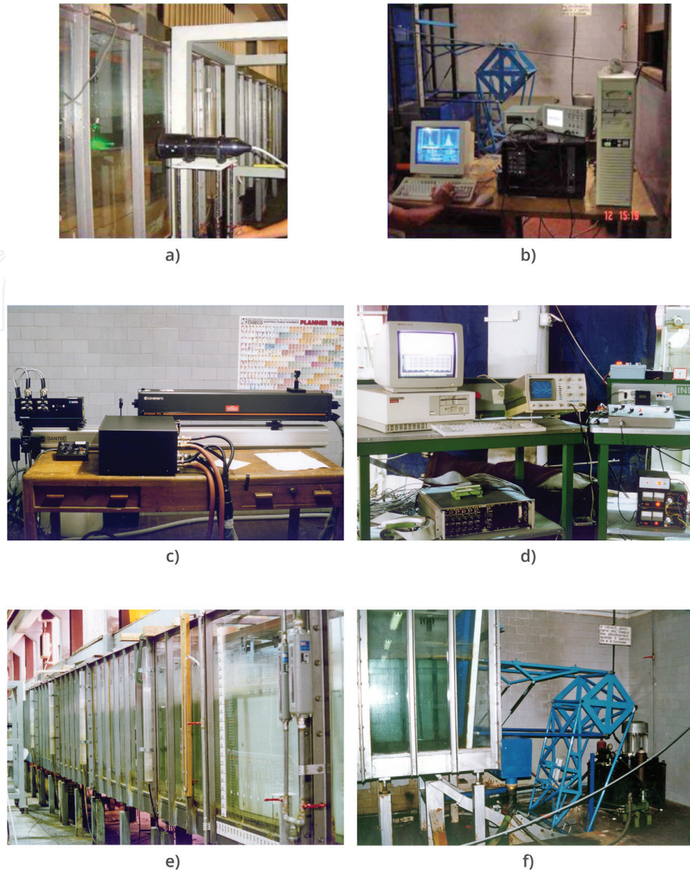
Figure 1. Experimental apparatus: (a) LDA probe; (b) DANTEC FVA signal processor and process computer; (c) laser coherent Innova and Dantec 2D fiber flow optics; (d) process computer with a AD/DA board for the wavemaker control; (e) a part of the wave channel; (f) the wavemaker.
