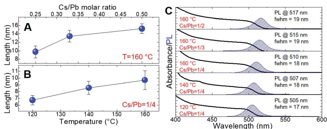
Fig. 3 (A) Behaviour of the nanocube length (deduced by TEM measurements) of the NCs synthesized at 160\text{ }^{\circ}\text{C} with different Cs/Pb molar ratios. (B) Behaviour of the nanocube length (deduced by TEM measurements) of the NCs synthesized with a Cs/Pb molar ratio of 1/4 at different temperatures. (C) UV-vis and PL spectra of the same nanocubes recorded in cyclohexane (only shown for the sample with near-unity PLQY).
