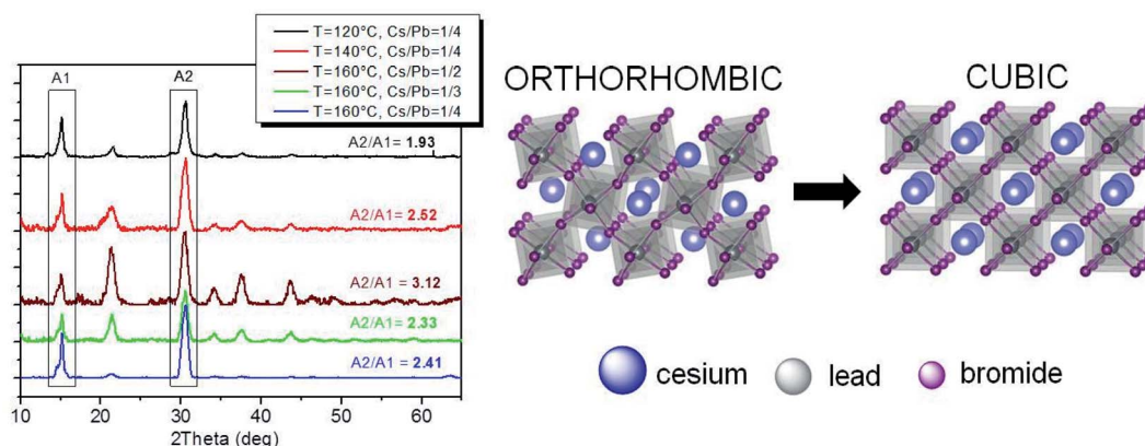
Fig. 7 (left) XRD experimental patterns ( \theta/2\theta scan and background subtracted) showing a higher preferred orientation for samples at 120^{\circ}\text{C} and 160^{\circ}\text{C} with \text{Cs/Pb} = 1/4 (black and blue curves, respectively). (right) A schematic representation of the orthorhombic and cubic structures of \text{CsPbBr}_3 differing for the tilting of \text{PbBr}_6^{4-} octahedra with respect to each other.
