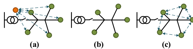
Fig. 8 Classification of grid-edge control strategies based on their communication network: a centralised control, b decentralised control, c distributed control. The green circles represent DERs, while the orange circle represents a central controller. The dashed blue lines represent two-way communication links
