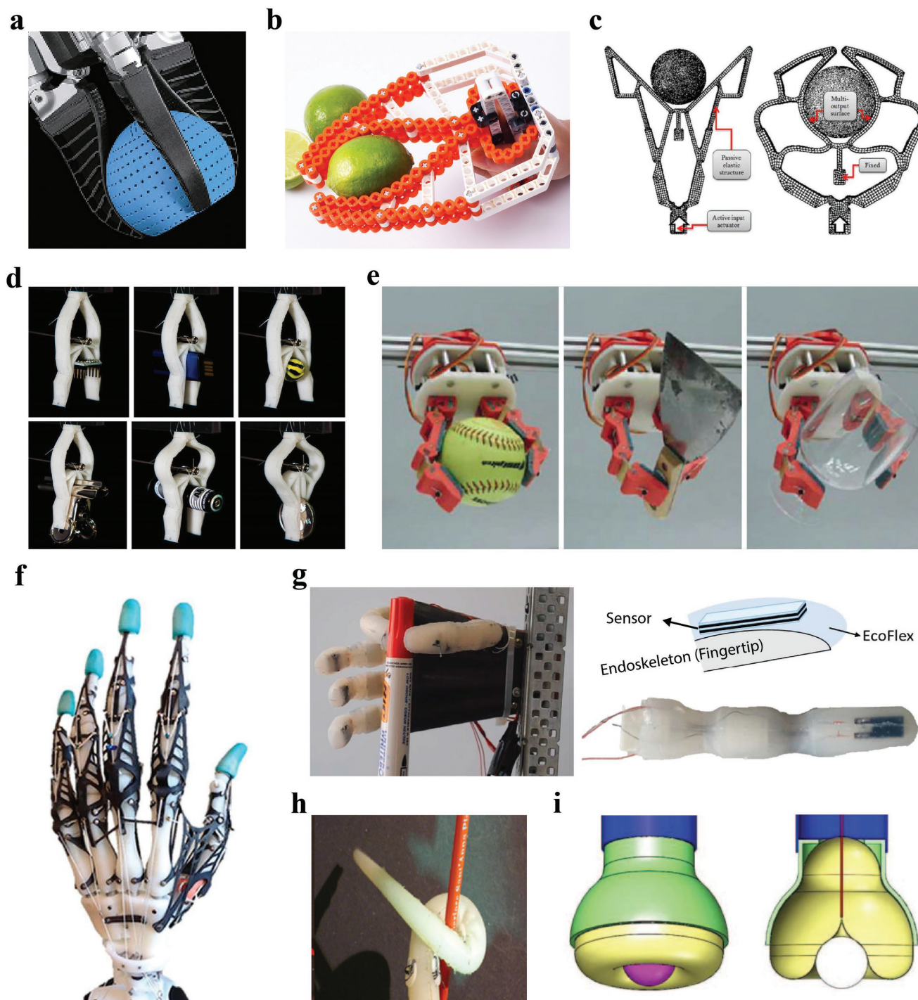
Figure 4. Soft grippers using passive structure with external motors. a) Fin Ray robotic gripper. [11] Reproduced with permission. Copyright Festo AG & Co. KG. b) Fin Ray (toy). Reproduced with permission. [6] Copyright BionicToys GmbH. c) Working principle of compliant mechanism. Reproduced with permission. [28] Copyright 2013, Emerald Publishing. d) Compliant mechanism. Reproduced with permission. [30] Copyright 2017, Springer Nature. e) Tendon-driven with elastic hinges. Reproduced with permission. [50] Copyright 2017, IEEE. f) Anthropomorphic tendon-driven. Reproduced with permission. [54] Copyright 2016, IEEE. g) Tendon-driven with sensor embedded soft skin. Reproduced with permission. [59] Copyright 2017, IEEE. h) Tendon-driven elastomeric manipulator. Reproduced with permission. [67] Copyright 2011, IOP Publishing. i) Tendon-driven with a compliant elastomeric bag. Reproduced with permission. [63] Copyright 2016, IEEE.
