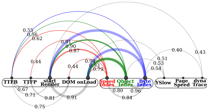
Figure 3: Arc diagram representing the correlation matrix between metrics pairs.
