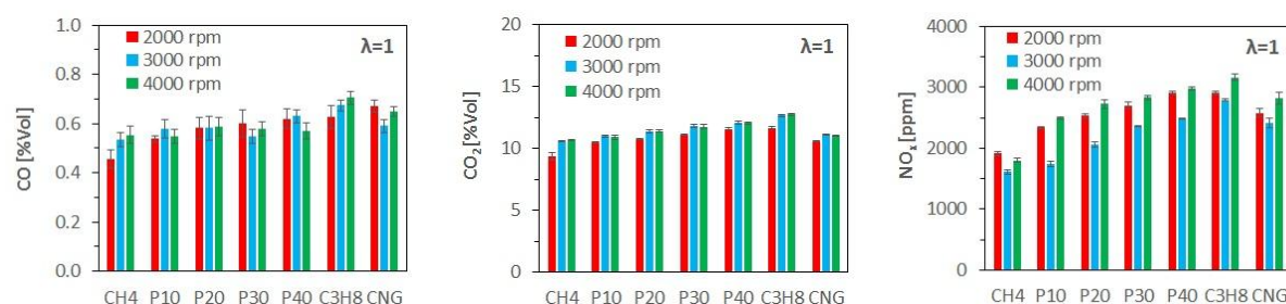
Figure 8. CO, CO 2 and NO x emissions for the three different engine speeds investigated.
