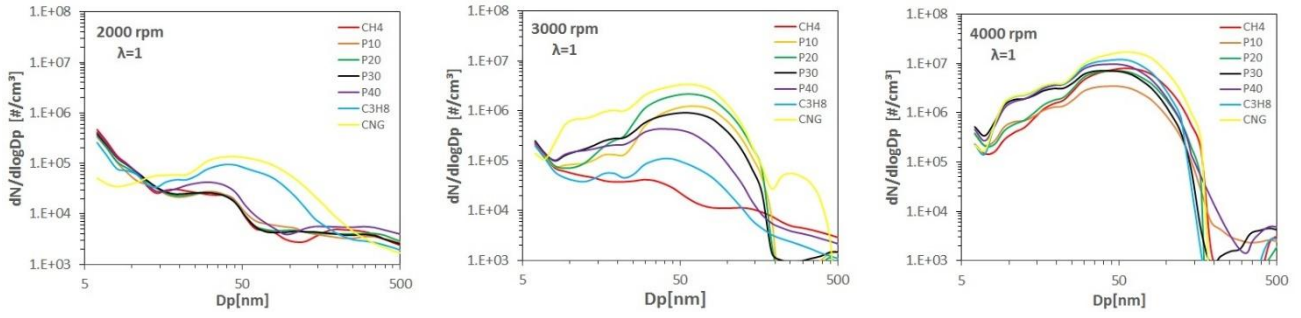
Figure 9. PSD functions for the three different engine speeds investigated.
