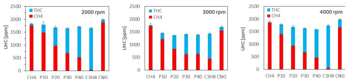
Figure 7. TUHC (blue bars) and CH 4 (red bars) emissions for the three different engine speeds investigated.
