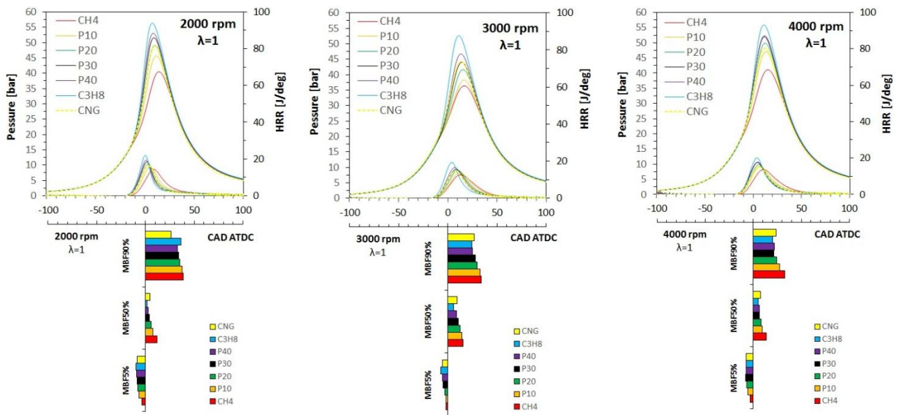
Figure 5. In-cylinder pressure, HRR, MBF5%, MBF50% and MBF90% for the three different engine speeds investigated.
