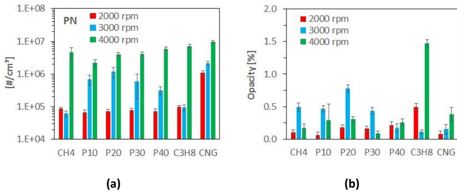
Figure 10. PN (a) and PM (b) for the three different engine speeds investigated.
