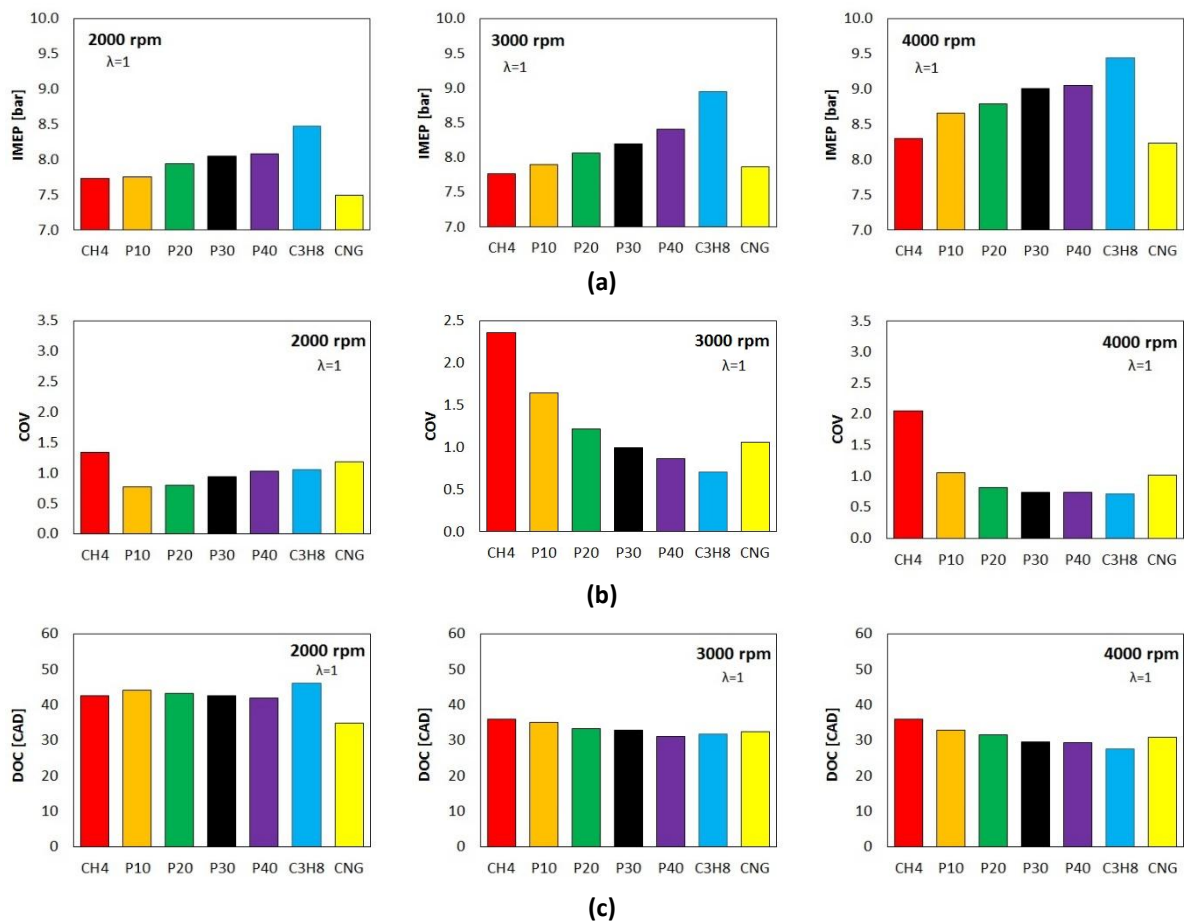
Figure 6. IMEP (a) COV (b) and DOC (c) for the three different engine speeds investigated.
