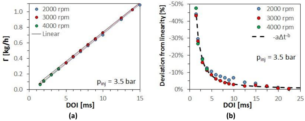
213 Figure 2. Measured mass flow rate \Gamma = \frac{f_{inj}^{ref}}{f_{inj}} \dot{m}_{exp} (a). Deviation from linearity due to injector mechanical delay (b).
