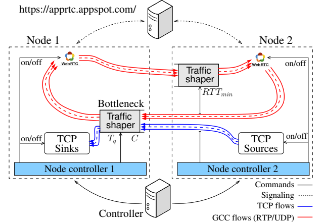
Figure 9. Experimental testbed
