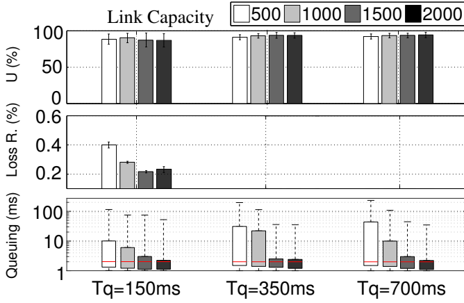
Figure 11. Channel utilization, Loss ratio and Queueing delay percentiles in the case of a single GCC flow over a bottleneck with different constant capacity C \in \{500, 1000, 1500, 2000\} kbps and bottleneck queue size \bar{T}_q \in \{150, 350, 700\} ms
