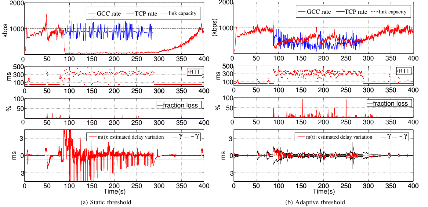
Figure 8. One GCC flow vs one TCP flow. Bottleneck parameters: queue size \bar{T}_q = 350\text{ms} , link capacity C = 1000\text{kbps}
