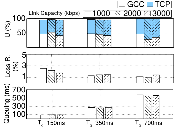
Figure 12. Channel utilization, Loss ratio and Queueing delay in the case of a GCC flow with a TCP flow over a bottleneck with different constant capacity C \in \{1000, 2000, 3000\} kbps and bottleneck queue size T_q \in \{150, 350, 700\} ms
