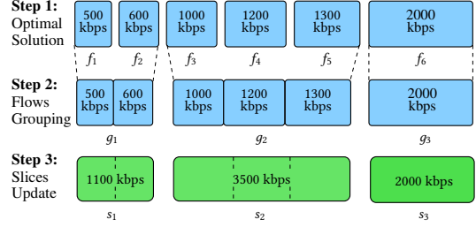
Fig. 5. The Quantized aggregation strategy
