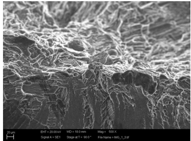
Fig. 16. Flat facets-to-dimple transition zone (500x).
