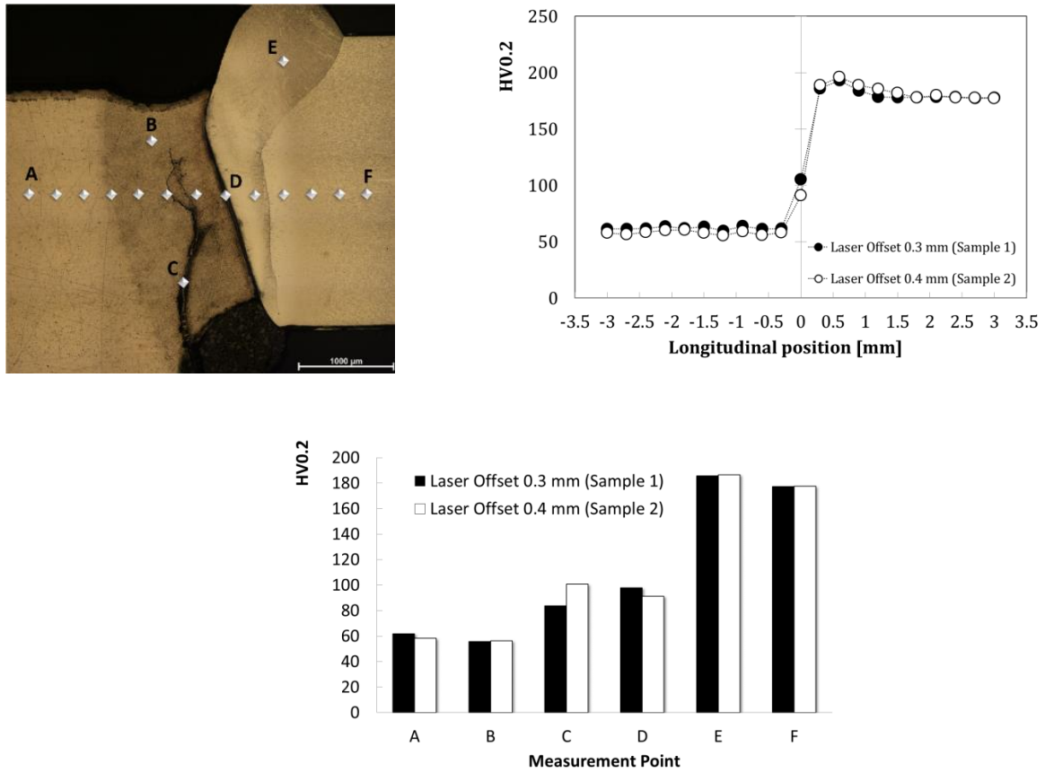
Fig. 7. Hardness profile and values along the weld in two different process conditions
