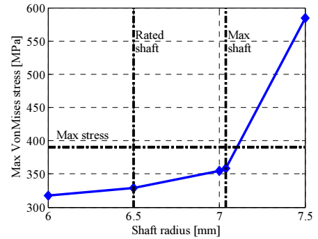
Figure 8 - Maximum stress as a function of shaft radius
