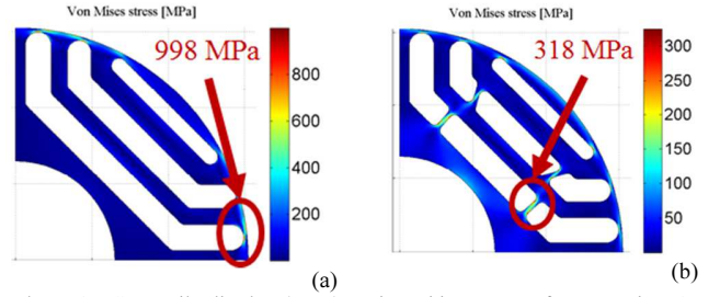
Figure 3 – Stress distribution (MPa) evaluated by means of structural FEA on preliminary (a) and final (b) rotor
