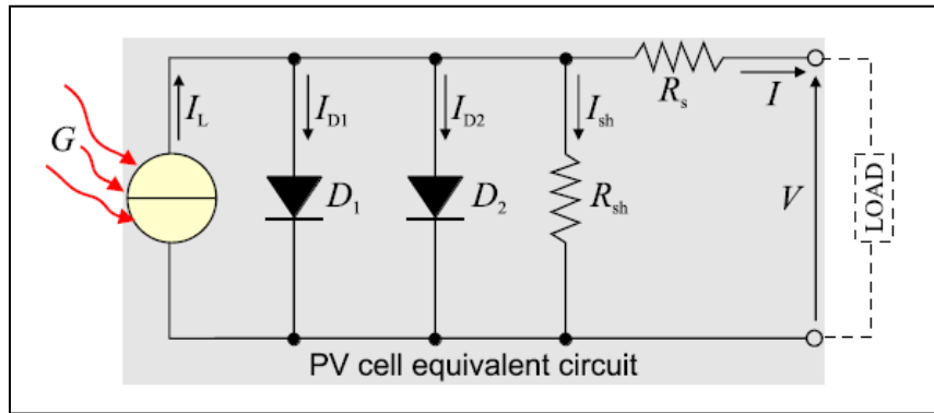
Fig.2 - Two diodes equivalent circuit of a PV cell
