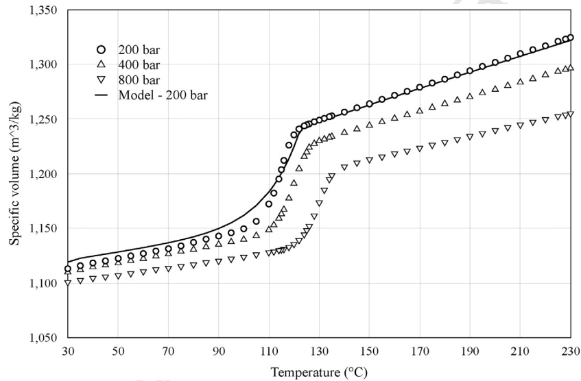
Fig. 3. pVT data with \dot{T}_0 = 5 °C/min.
