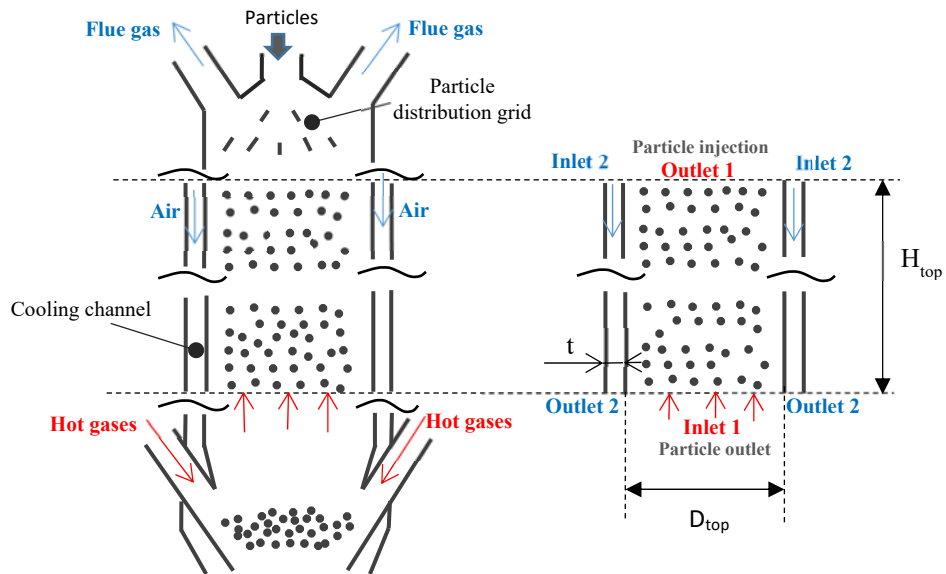
Figure 4. Architecture for the top column (left) and simulated part (right) (design parameters: H_{top} and D_{top} ; fixed parameter: t=0.06\text{m} )
