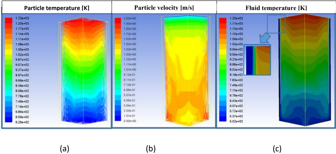
629 630 (a) (b) (c) 631 Fig. 12. Particle temperature (a), particle velocity (b) and air temperature (c) of individual 2302 (bottom 632 column) 633
