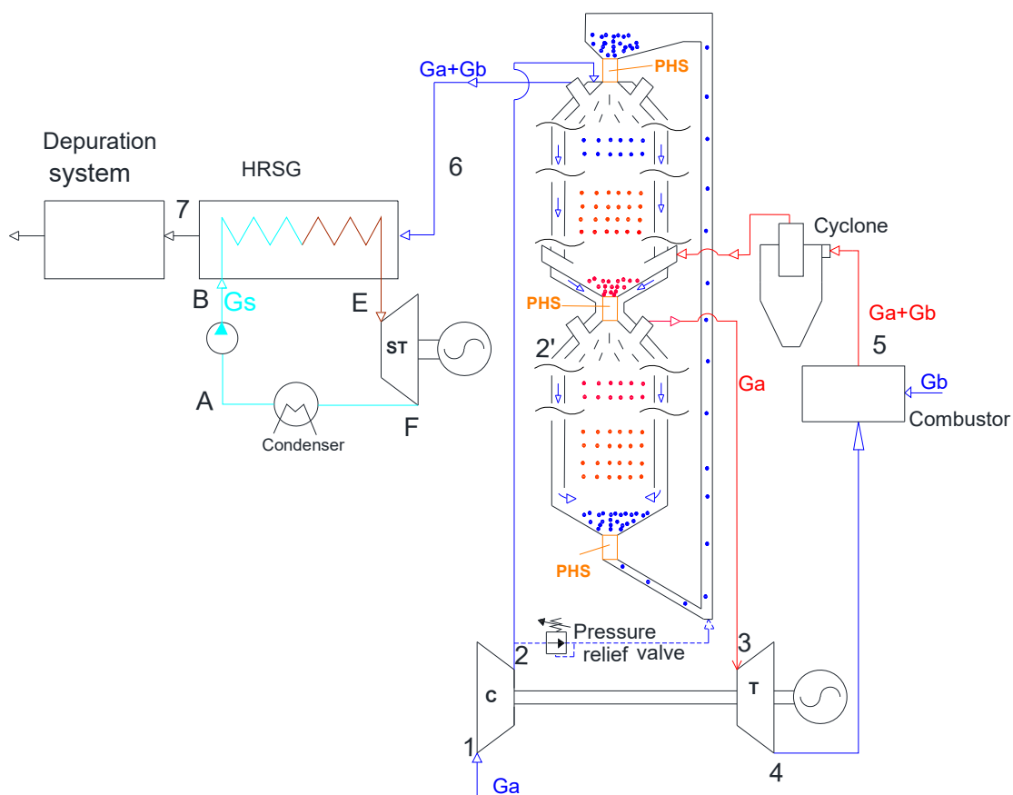
Fig.2. Application of the IPHE to small scale combined cycles (PHS= particle handling systems, HRSG=heat recovery steam generator, G_a = air mass flow rate, G_b = fuel mass flow rate, G_s =steam mass flow rate)
