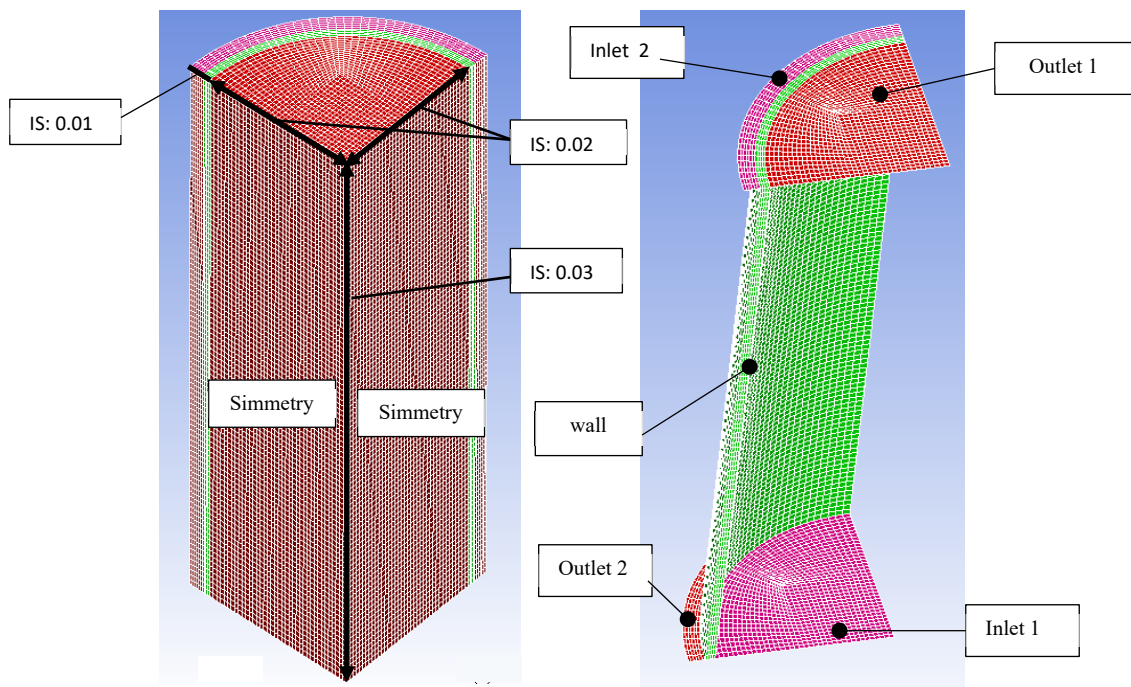
Fig. 5. Computational grid employed for the top column, example for D_{top}=1.5\text{ m} and H_{top}=3\text{m} . (IS=interval size expressed in meters)
