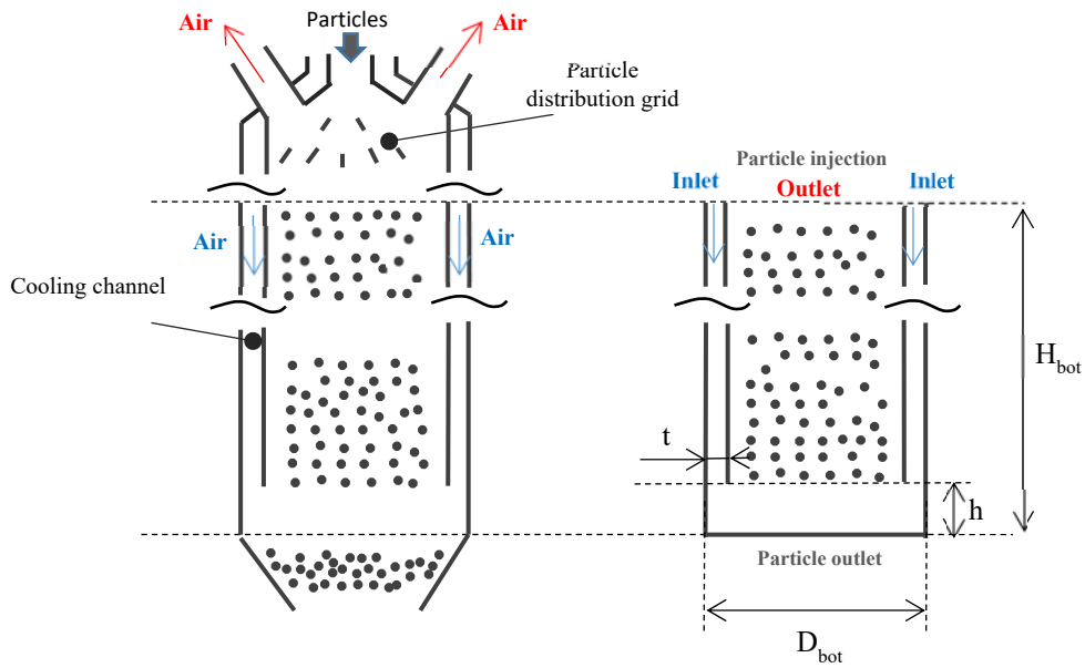
Fig. 6. Architecture for the bottom column (left) and simulated part (right) (design parameters: H_{bot} and D_{bot} ; fixed parameters: t=0.06m and h=0.3m )
