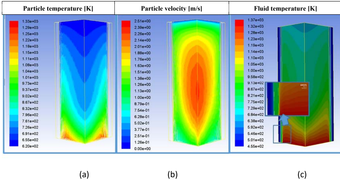
Fig. 12. Particle temperature (a), particle velocity (b) and gas temperature (c) of individual 2302 (top column)
