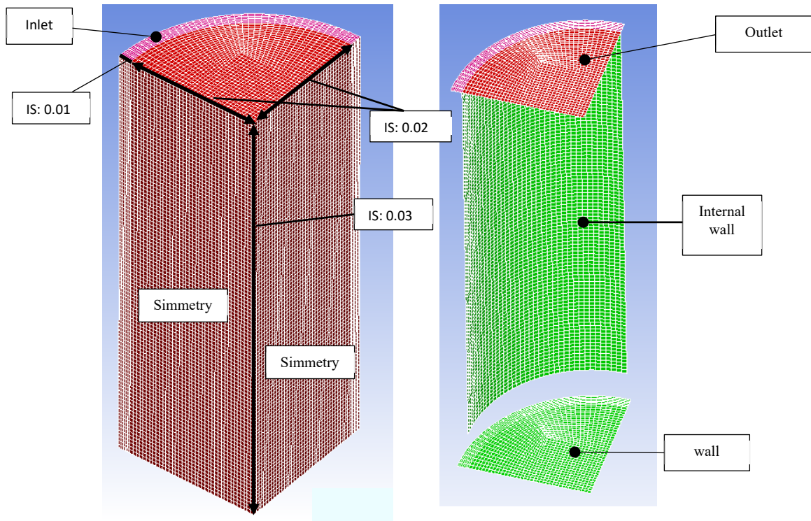
Fig. 6. Architecture for the bottom column (left) and simulated part (right) (design parameters: H_{bot} and D_{bot} ; fixed parameters: t=0.06m and h=0.3m )
