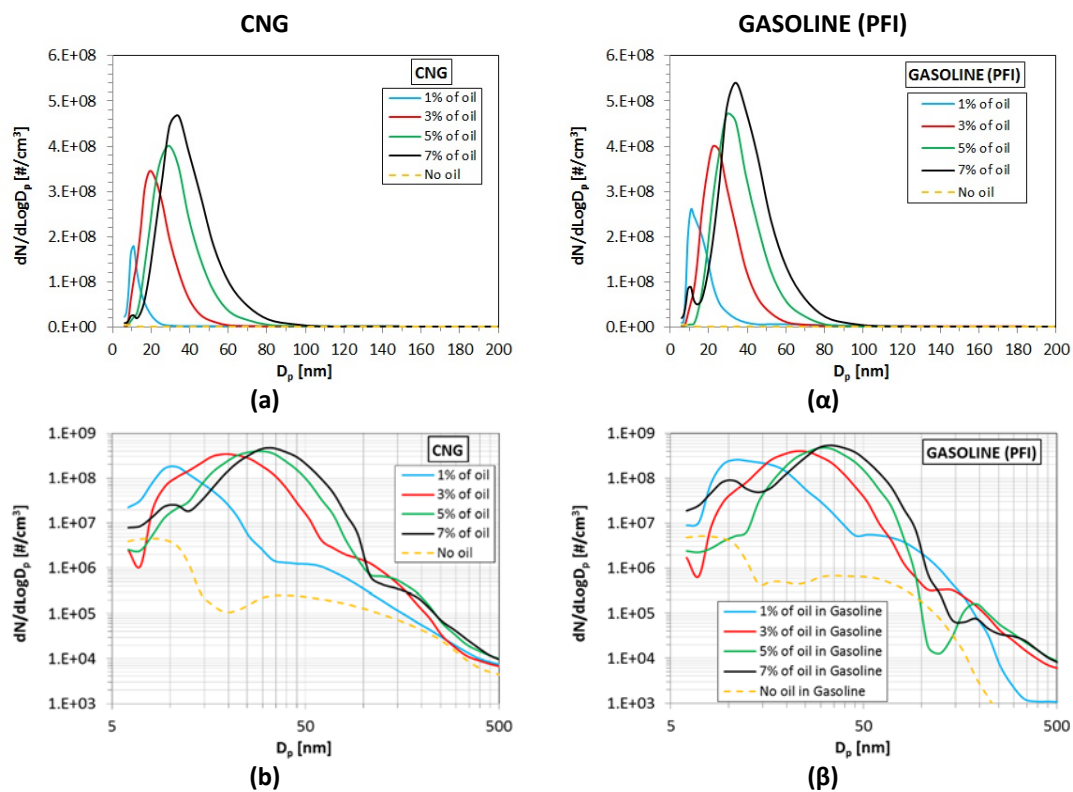
Figure 7 PSD functions (mean values) with a mass lubricant oil content equal to 0% (yellow line), 1% (light blue line), 3% (red line), 5% (green line) and 7% (black line), for both the CNG (Latin characters) and gasoline (Greek characters) PFI tests. For clarity, the data are plotted by using both a linear (a) and (α), and a logarithmic scale (b) and (β).
