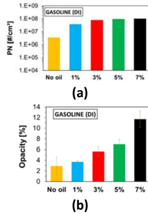
Figure 11 Total concentration number (a) and opacity [%] (b) for gasoline DI tests.
