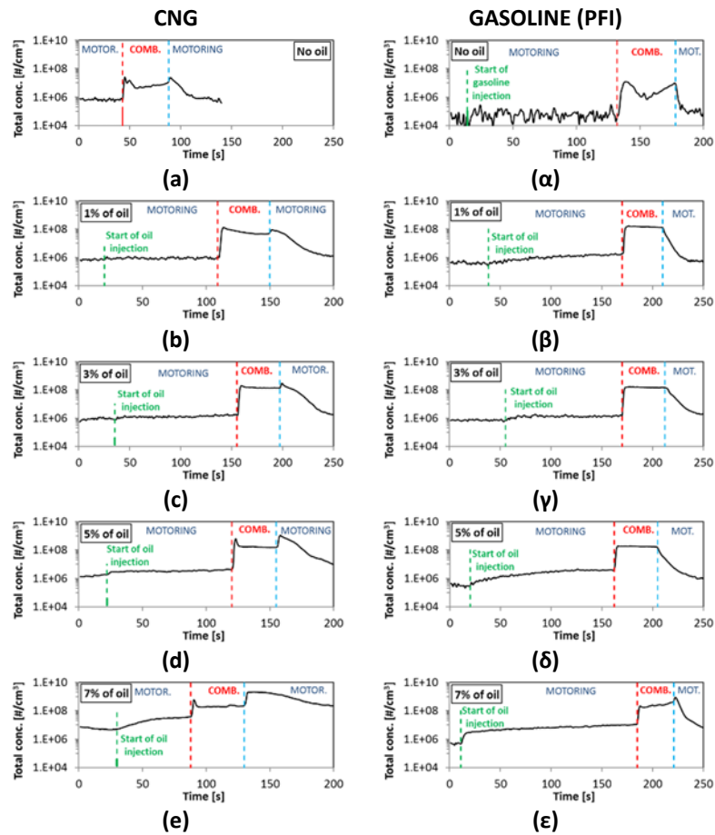
Figure 5 Total concentration number trace evolution with time of one representative case for each explored operating condition, for both the CNG (Latin characters) and gasoline (Greek characters) PFI tests. Green dashed line: start of oil injection into the intake manifold; red dashed line: start of combustion; light blue dashed line: end of combustion.
