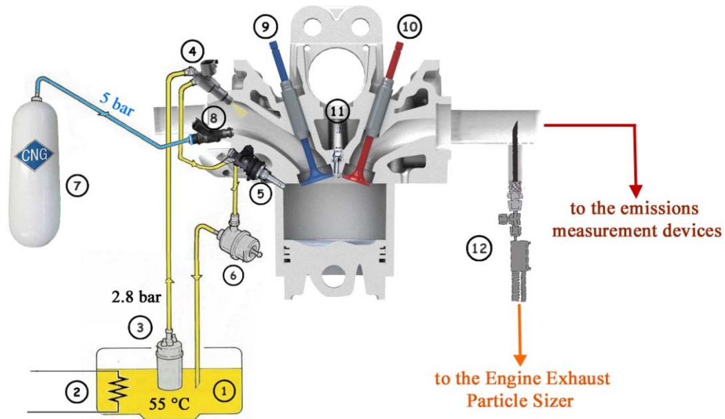
Figure 1. Experimental Set-up for the CNG tests. (1) Oil tank; (2) resistors for heating the oil to 55 °C; (3) oil pump; (4) 3-hole commercial low pressure injector; (5) 6-hole commercial high-pressure injector; (6) oil pressure regulator; (7) CNG bottle; (8) CNG 1-hole injector; (9) intake and (10) exhaust valves; (11) spark-plug; (12) particle sizer probe.
