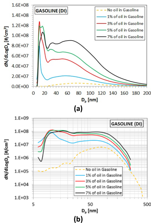
Figure 10 PSD functions (mean values) with mass lubricant oil content equal to 0% (yellow line), 1% (light blue line), 3% (red line), 5% (green line) and 7% (black line). For clarity, the data are plotted by using both a linear (a) and a logarithmic scale (b).
