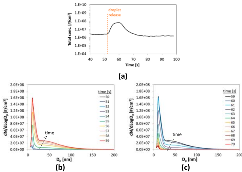
Figure 12 Total concentration number trace evolution with time (a) and PSD time evolution during the first 9 seconds (b) and the subsequent 10 seconds (c), for emulsion of oil droplet release.
