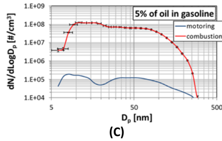
Figure 9 Statistical PSD functions (a), total concentration number trace evolution with time (b) and PSD functions during motoring conditions and combustion (c) of one representative case (5% of oil) for gasoline DI tests.
