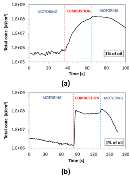
Figure 3 Total PN concentration measurements for CNG test with 1% of oil without (a) and with (b) “film-strategy”. Red dashed line: start of combustion; light blue dashed line: end of combustion.
