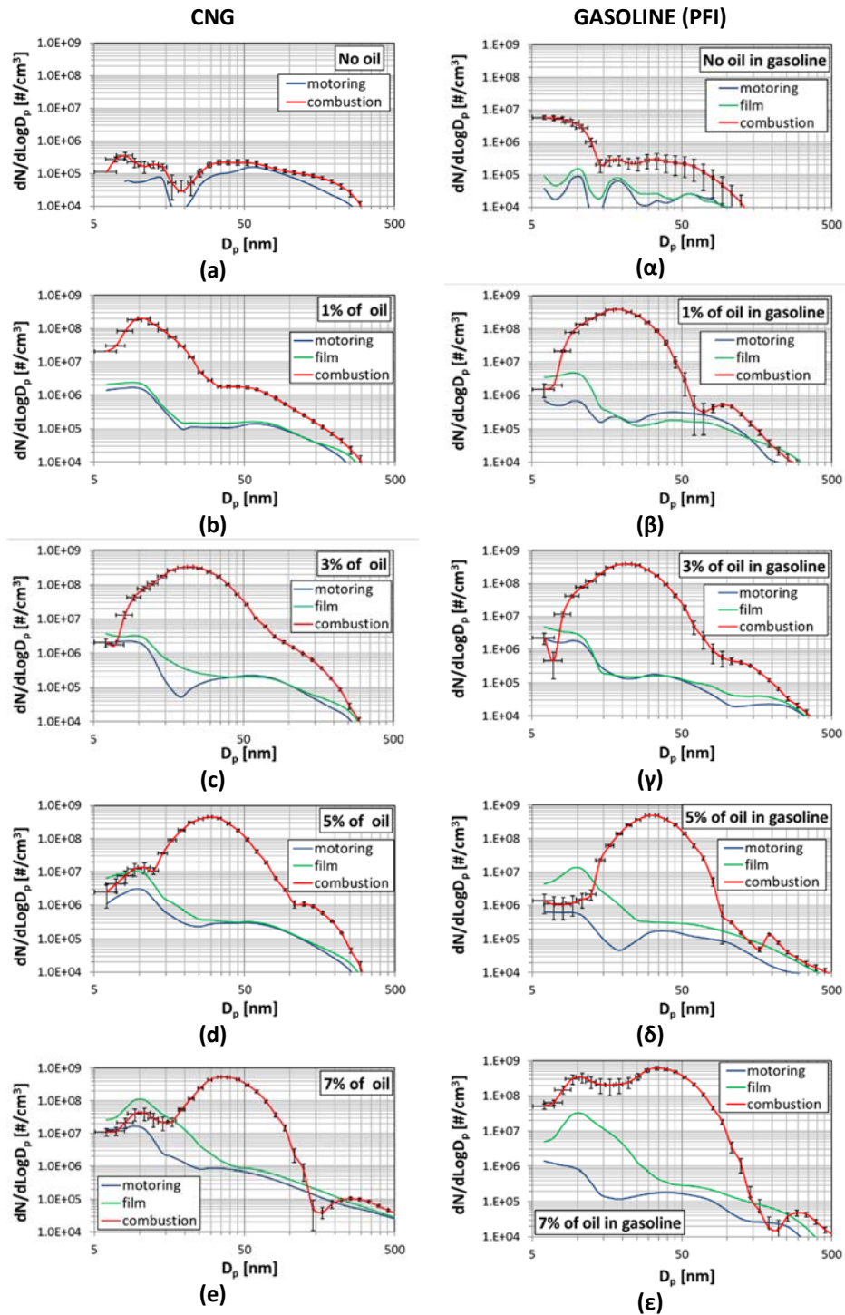
12 Figure 6 PSD functions for one representative case for each explored operating condition for both the CNG (Latin 13 characters) and gasoline (Greek characters) PFI tests. Light blue line: PSD during motoring conditions; green line: PSD 14 after film forming; red line: PSD during combustion
