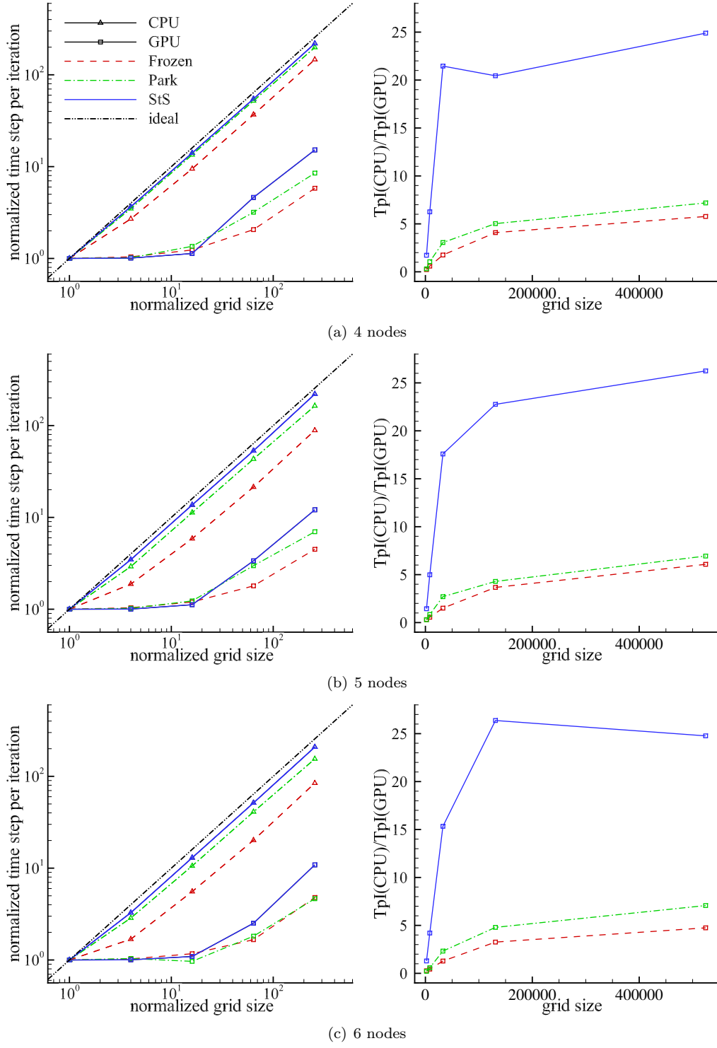
Fig. 13: Performance results obtained by using full node computational power (each node has 12 CPU cores and 2 GPUs cards): (left) time per iteration (Tpl) normalized by the one obtained on the coarsest grid as a function of the grid size normalized by the coarsest grid size. (right) \text{Tpl}(\text{CPU})/\text{Tpl}(\text{GPU}) as a function of the grid size.
