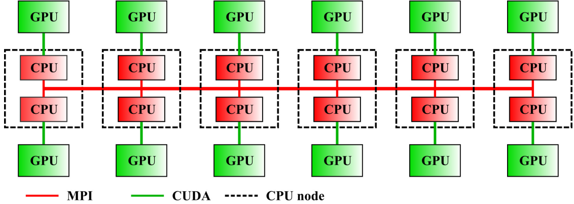
Fig. 1: Scheme of the GPU cluster along with the MPI-CUDA paradigm (based on Su et al. [38])
