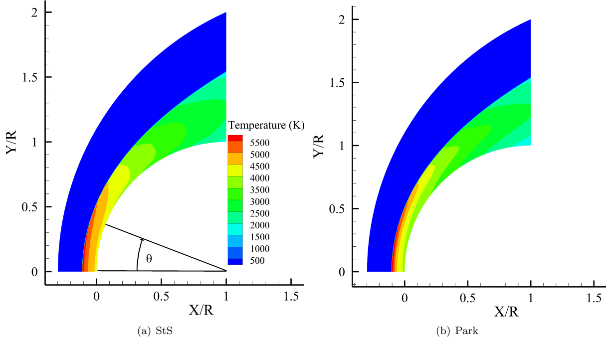
Fig. 8: Translational temperature contour plot: (a) StS; (b) Park.
