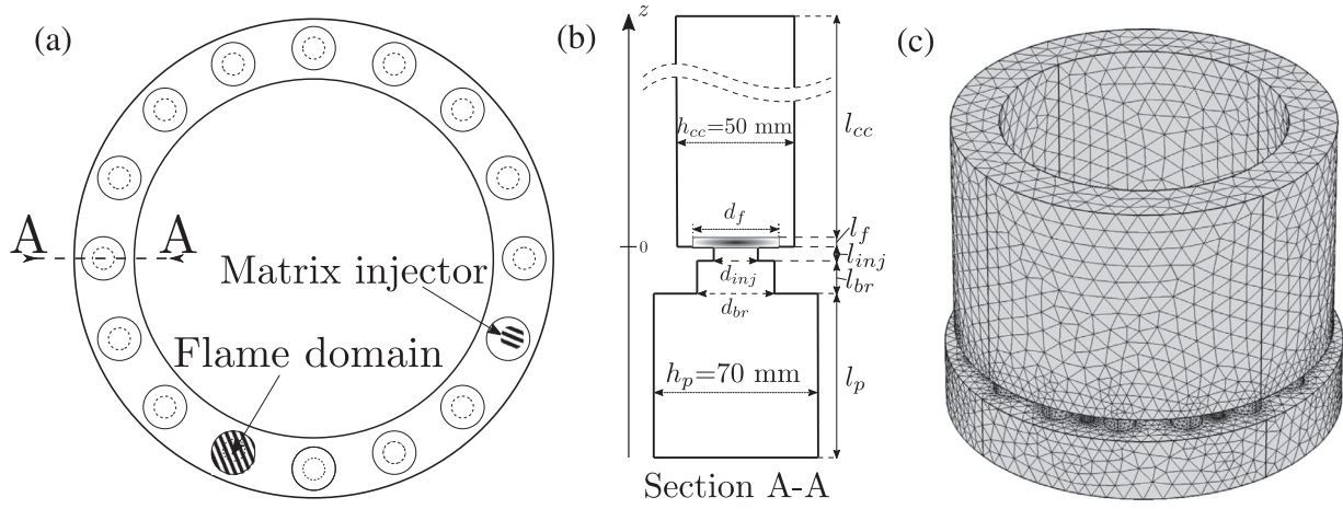
Fig. 3. (a) Top view schematic representation of the model. (b) Longitudinal A-A cut showing geometrical details of the matrix injector model and of the flame domain. (c) Three dimensional model of the MICCA chamber with the details of the unstructured mesh comprising approx. 130,000 tetrahedral elements.
