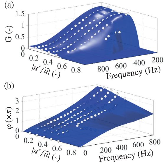
Fig. 5. Interpolated Flame Describing Function (FDF) obtained for operating point A: \phi=1.00 and u_b=0.49 \text{ ms}^{-1} . Experimental data points are displayed as white dots. (a) Gain. (b) Phase \varphi .
