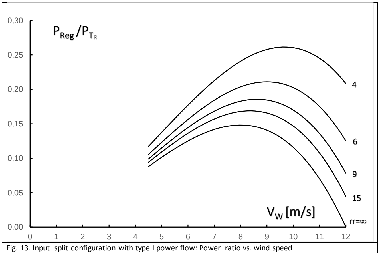
Fig. 13: Input split configuration with type I power flow: Power ratio vs. wind speed
