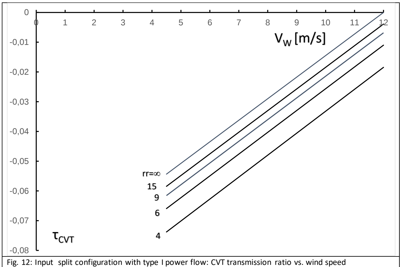
Fig. 12: Input split configuration with type I power flow: CVT transmission ratio vs. wind speed
