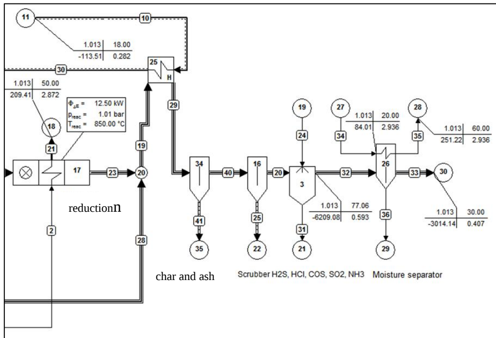
Figure 5 Last part of the gasifier model
