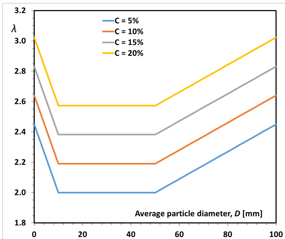
Figure 10 Equivalence ratio, \lambda , vs. average particle diameters, D , at constant ash content, C
