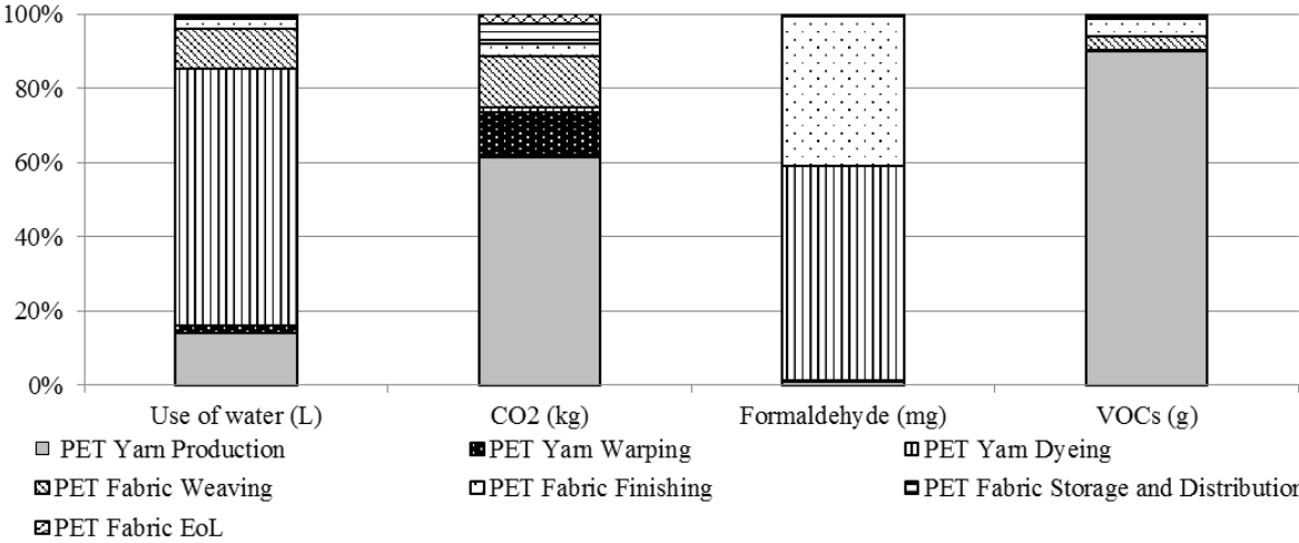
Fig. 2 Inventory results, elementary flows: Use of water, CO 2 , Formaldehyde, VOCs.
