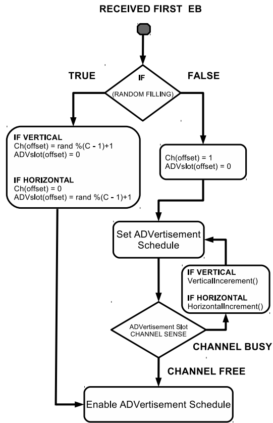
Figure 3: Joining Algorithm.
