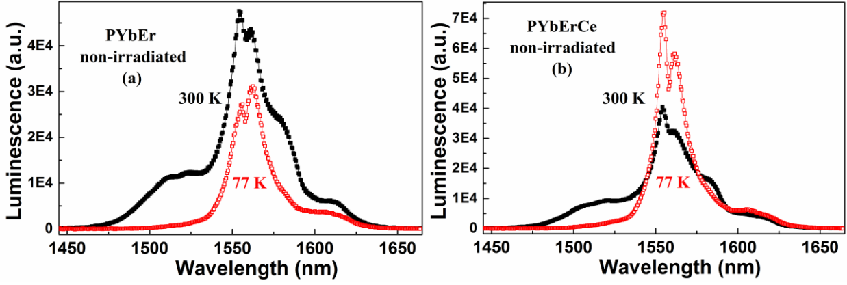
Fig. 9: Luminescence intensity spectra at RT (black squares) and LT (77 K, empty red squares) temperature (a) for PYbEr sample without \text{Ce}^{3+} -doping and (b) for PYbErCe sample with \text{Ce}^{3+} -doping.
