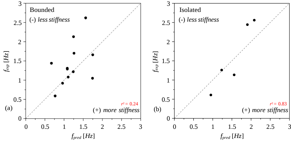
Figure 8. Comparison between experimental and estimated first natural frequency for the Spanish Standards NCSE 2002: (a) bounded, (b) isolated.
