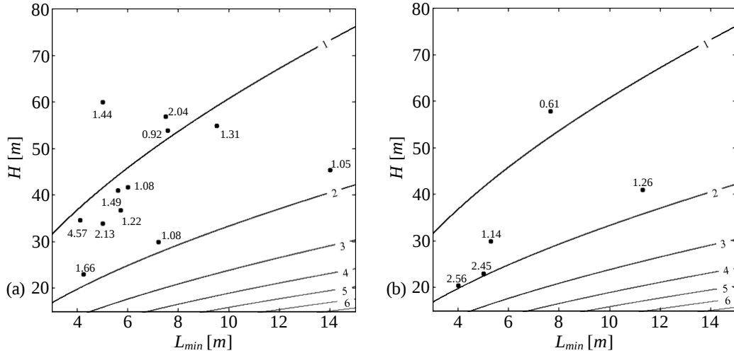
Figure 6. Development of iso-frequency curves based on the Spanish Standards NCSE 2002: (a) bounded tower, (b) isolated towers. The “dots” are relative to the experimental frequencies.
