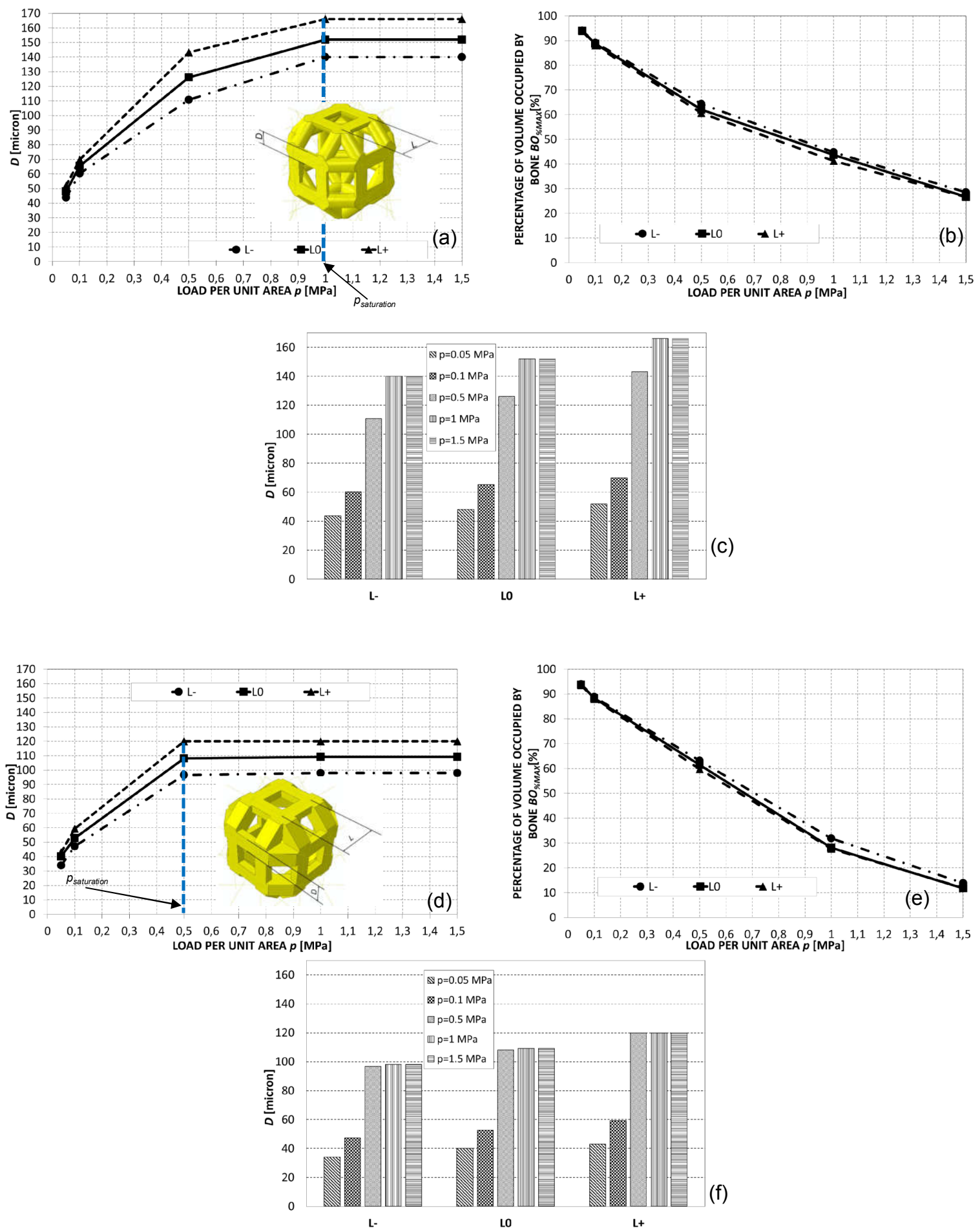
Fig. 9. Values of D (a, d) and BO_{\%MAX} (b, e) predicted by the algorithm for different values of L in the case of circular (a, b) and square (d, e) cross-section. Values of D expressed in function of the dimension L for the circular (c) and square (f) cross-section. Increasing values of L lead to increasing values of D , which is consistent with the physics of the problem. In fact, as L increases, the global scaffold stiffness decreases. Therefore, in order to re-establish the original scaffold stiffness, the algorithm increases the dimension D . For the sake of brevity, only the results referring to E = 1000 MPa are shown in the figure.
