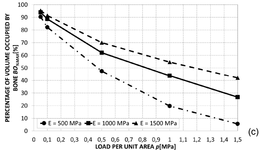
Fig. 6. Optimization of the rhombicuboctahedron unit cell, circular cross-section. (a) Optimal scaffold geometries predicted by the algorithm, in the case of circular cross-section. Values of the optimal diameter D (b) and of BO_{\%MAX} (c) predicted by the algorithm for different levels of load and scaffold Young's modulus. For the sake of clarity, the only saturation load p_{saturation} related to E = 500 MPa is shown in the figure.
