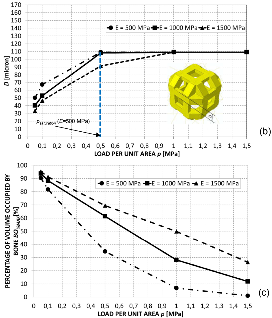
Fig. 7. Optimization of the rhombicuboctahedron unit cell, square cross-section. (a) Optimal scaffold geometries predicted by the algorithm, in the case of square cross-section. Values of the optimal diameter D (b) and of BO_{\%MAX} (c) predicted by the algorithm for different levels of load and scaffold Young's modulus. For the sake of clarity, the only saturation load p_{saturation} related to E = 500 MPa is shown in the figure.
