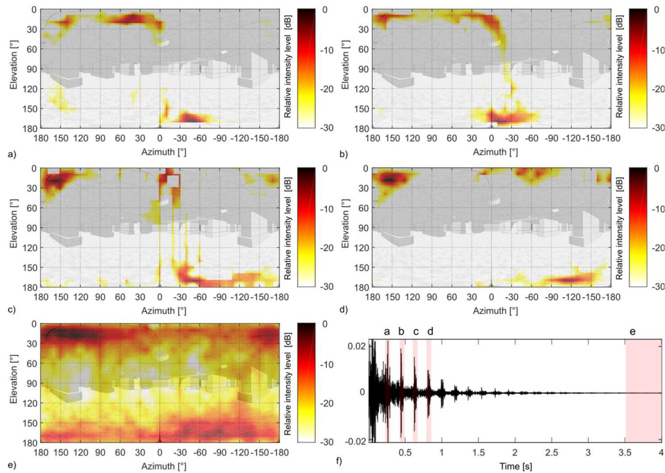
Fig. 9. Comparison between directional reflection maps at 500 Hz for combination S2-R11 at: a) 0.259 s from direct sound 50 ms time window; b) 0.438 s from direct sound 50 ms time window; c) 0.620 s from direct sound 50 ms time window; d) 0.805 s from direct sound 50 ms time window; e) 3.50 s from direct sound 0.5 s time window. f) Impulse response (omnidirectional) with shaded areas indicating the time intervals used in panels a-e). IR amplitude is expressed using arbitrary units.
