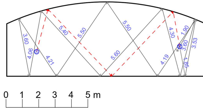
Fig 12. Schematic geometrical acoustic interpretation of the flutter echo appearing between source S2 and receiver R11. (---) propagation from source (S) to receiver (R), (—) roundtrip from (R) to (R).
