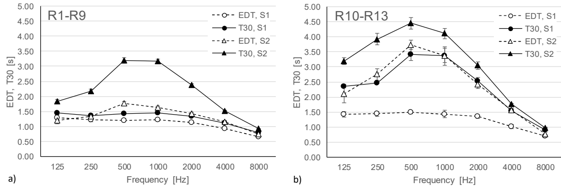
Fig. 4. Graphs of EDT and T30 values as a function of frequency and source position and receiver location: a) average of receivers located in the galleries (R1-R9); b) average of receivers located in the rotunda (R10-R13). Error bars correspond to standard deviation across measured values.
