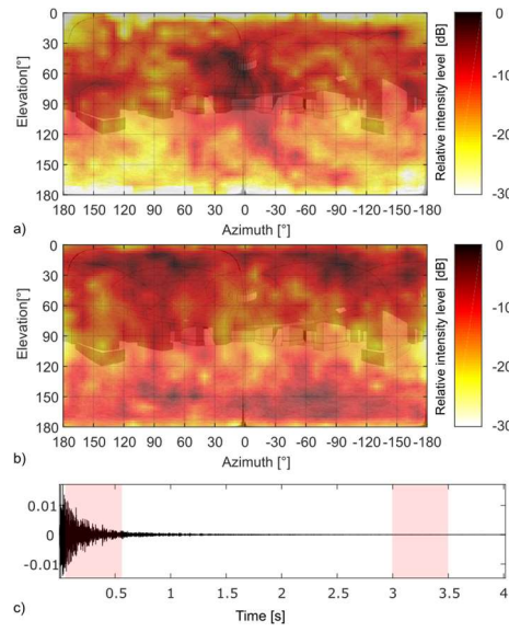
Fig. 10. Comparison between directional reflection maps at 500 Hz for combination S1-R11 at: a) 50 ms from direct sound 0.5 s time window; b) 3.0 s from direct sound 0.5 s time window. c) Impulse response (omnidirectional) with shaded areas indicating the time intervals used in a) and b). IR amplitude is expressed using arbitrary units.
