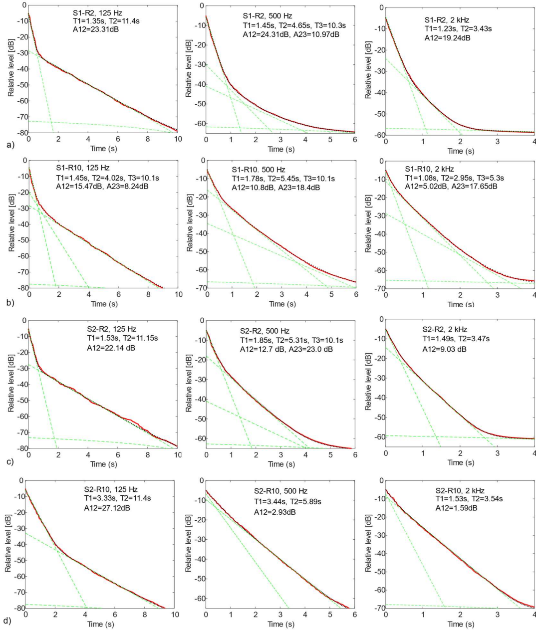
Fig. 6. Results of Bayesian analysis applied to 125 Hz, 500 Hz, and 2 kHz octave bands, at combinations: a) S1-R2; b) S1-R10; c) S2-R2; d) S2-R10. (—) Measured decay; (...) Bayesian decay; (- - -) Bayesian decay components.
