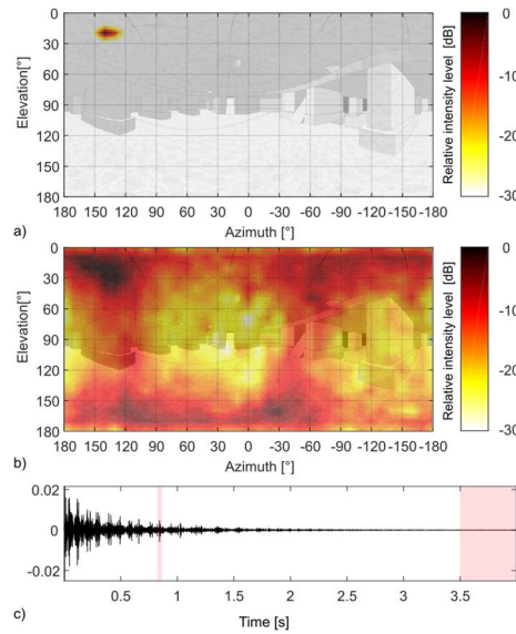
Fig. 8. Comparison between directional reflection maps at 500 Hz for combination S2-R10 at: a) 0.840 s from direct sound 10 ms time window; b) 3.50 s from direct sound 0.5 s time window. c) Impulse response (omnidirectional) with shaded areas indicating the time intervals used in a) and b). IR amplitude is expressed using arbitrary units.
