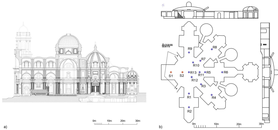
Fig. 2. a) Longitudinal sections of the cathedral and its crypt. b) Schematic plan and cross-sections of the crypt, with indication of source (S) and receiver (R) locations.
