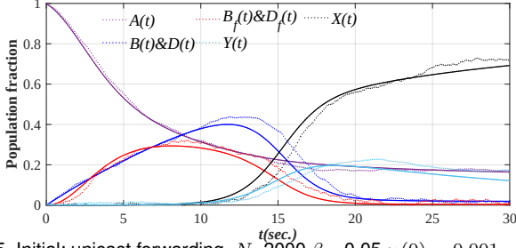
Fig. 5. Initial: unicast forwarding, N=2000, \beta_k=0.05, y(0) = 0.001
