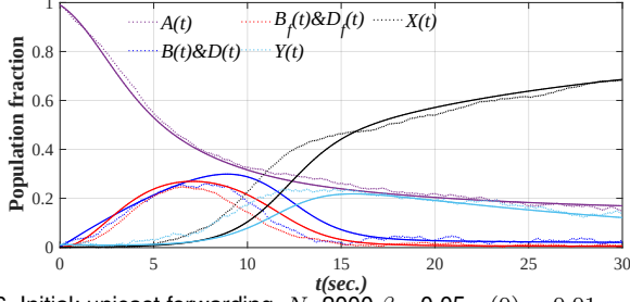
Fig. 6. Initial: unicast forwarding, N=2000, \beta_k=0.05, y(0) = 0.01
