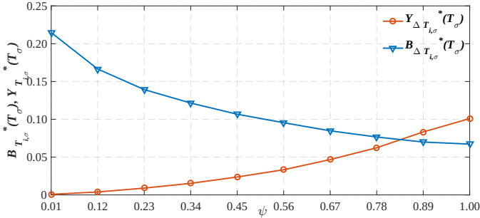
Fig. 9. The value of B_{T_{i,\sigma}}^*(T_\sigma) and Y_{T_{i,\sigma}}^*(T_\sigma) vary with \psi
