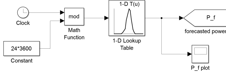
Figure 9: The Simulink model of wind and photovolac sources.
