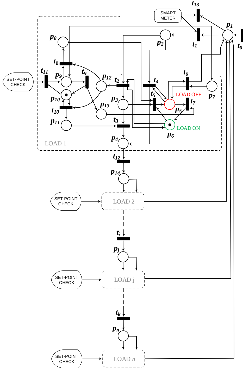
Figure 10: The load controller model.
