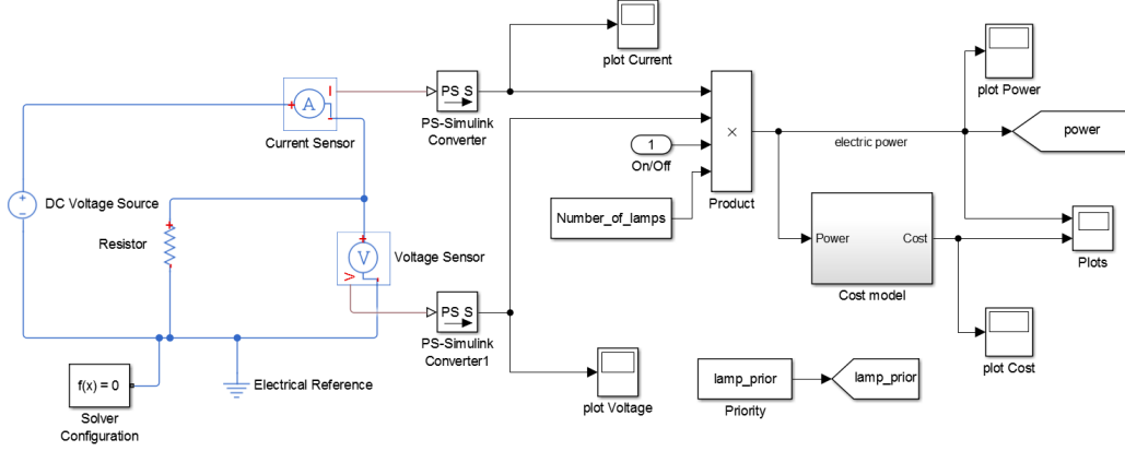
Figure 7: The Simulink model of the dimmable lamps.
