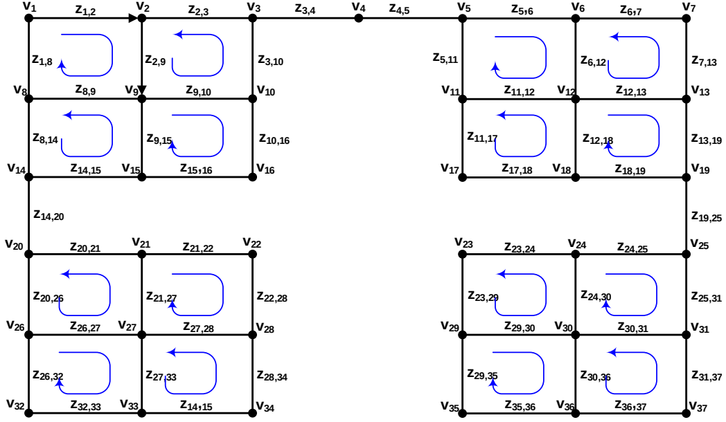
Figure 4: The guided path network of the example.
