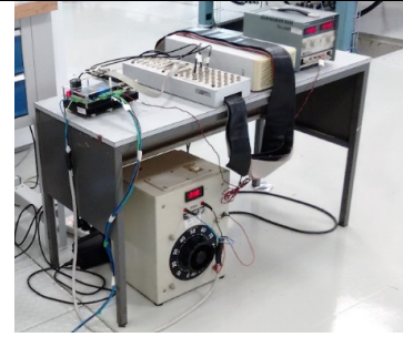
Fig. 5 - Motor Control Set-up
