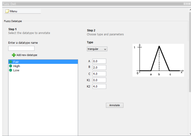
Fig. 5 (a) Individuals Tab, (b) Creation of a fuzzy datatype Fair with the Fuzzy Owl plug-in.
