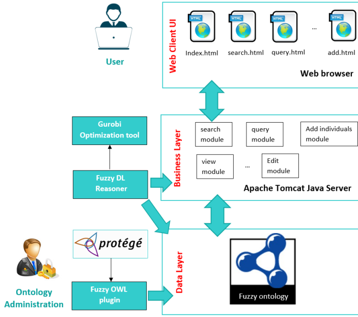
Fig. 3 Model of our tool, and linked components.
