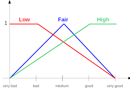
Fig. 2 The fuzzy sets we use to deal with Non-Functional Requirements.
