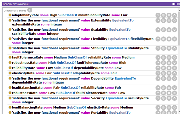
Fig. 6 General class axioms Tab.
