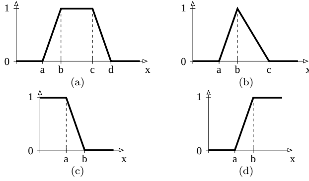
Fig. 1 (a) Trapezoidal function trz(a, b, c, d) , (b) triangular function tri(a, b, c) , (c) left shoulder function ls(a, b) , and (d) right shoulder function rs(a, b) .
