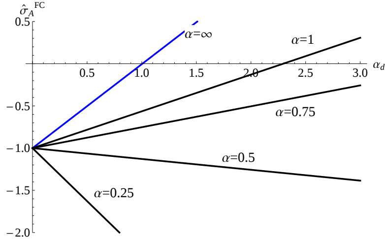
Fig.5. Tension to jump into full-contact \hat{\sigma}_A^{FC} as a function of parameter \alpha_d for various roughness parameter \alpha = 0.25, 0.5, 0.75, 1, \infty . The case \alpha = \infty (blue solid line) corresponds to the smooth dimple, whereas for the cases of small \alpha < 0.57 we have taken an upper bound estimate considering the value reached at \hat{c} = 1 , as otherwise the actual minimum depends on the details of the system, see also "Discussion".
