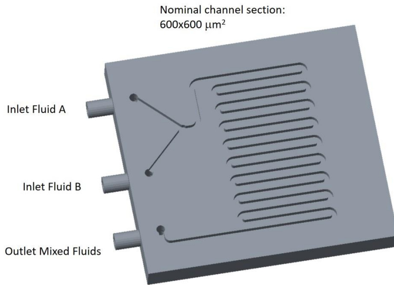
Figure 1 The analyzed AM microdevice (courtesy of Prof. Filippini)
