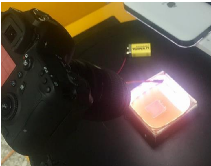
Figure 3 Experimental set-up
