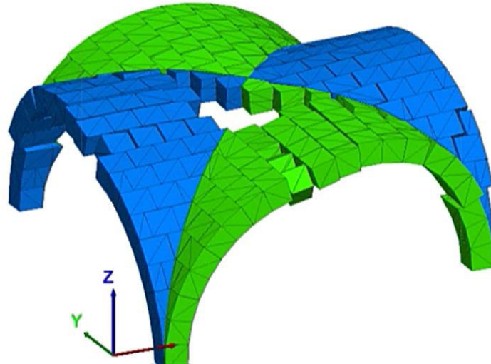
Figure 15. Vertical collapse test: Limit state before collapse.
