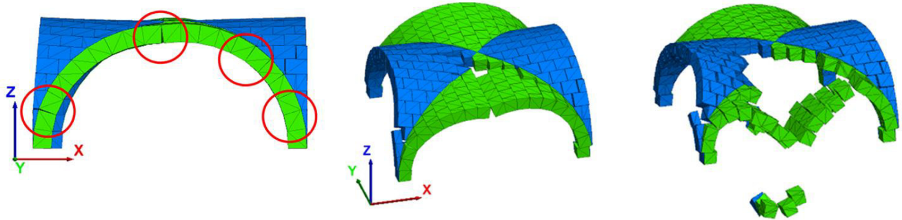
Figure 3. Displacement in x-direction: damage mechanism.
