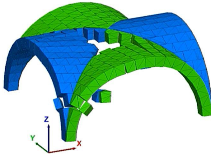
Figure 17. Diagonal collapse test: Limit state before collapse.
