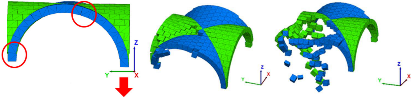
Figure 5. Vertical displacement: damage mechanism.
