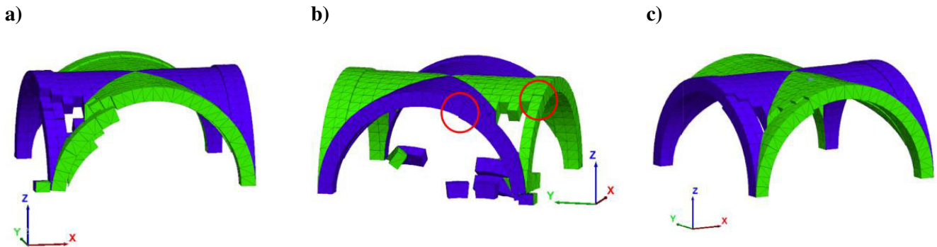
Figure 6. Damage mechanisms: a) horizontal (x-direction), b) diagonal (xy-direction) and c) vertical.
