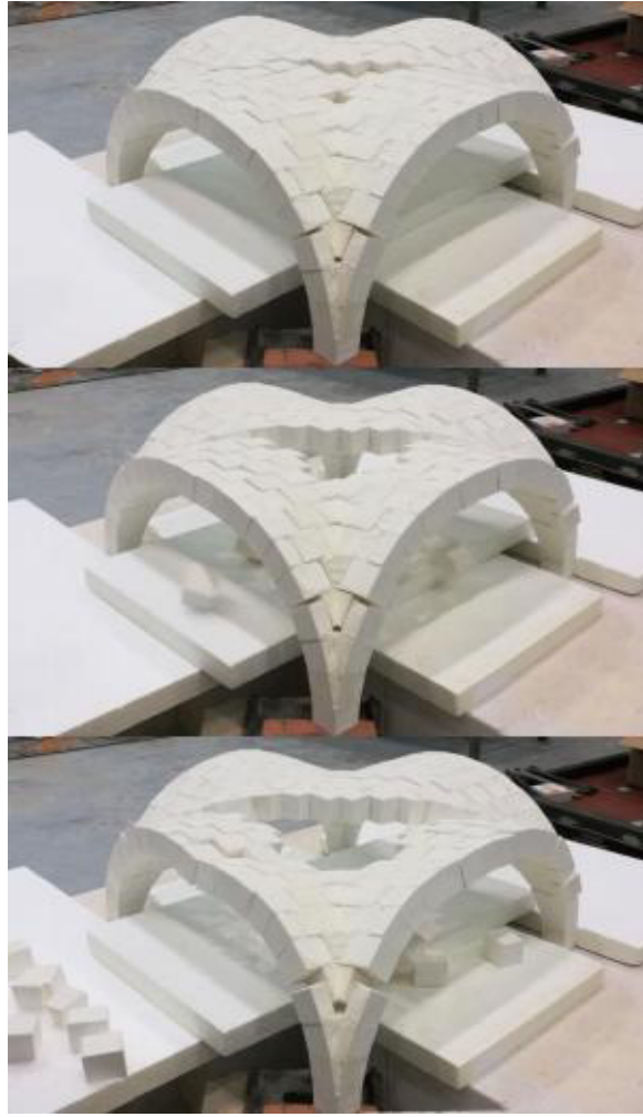
Figure 14. Diagonal collapse test: collapse mechanism.
