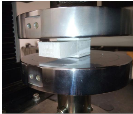
Fig.9 Test Structure.
