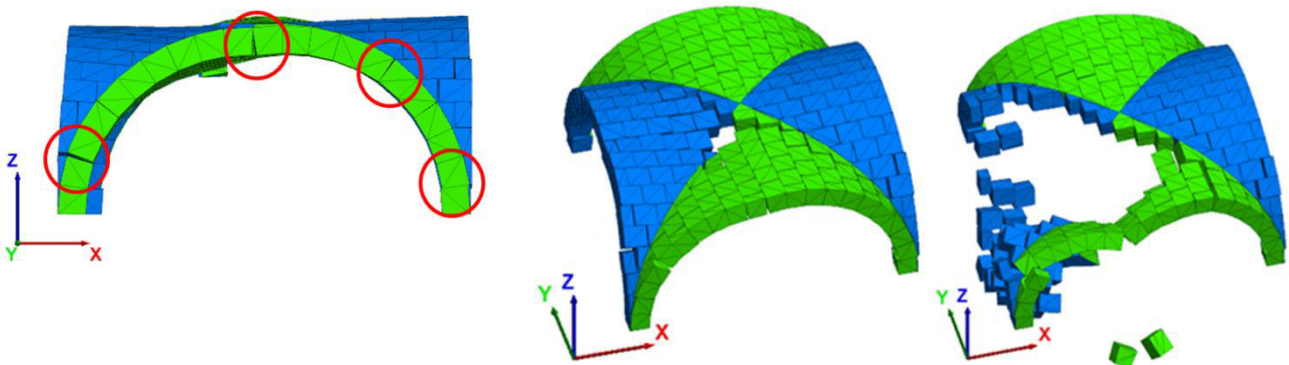
Figure 4. Diagonal displacement in xy-direction: damage mechanism.
