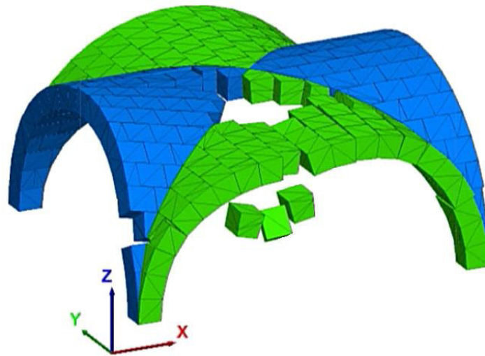
Figure 16. Horizontal direction collapse test: Limit state before collapse.
