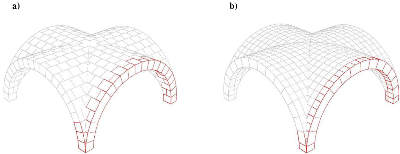
Figure 2. Computational model with a) orthogonal weaving and b) parallel weaving.
