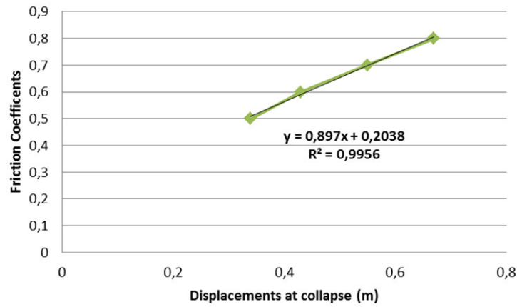
Figure 7. Displacements for different friction coefficients.
