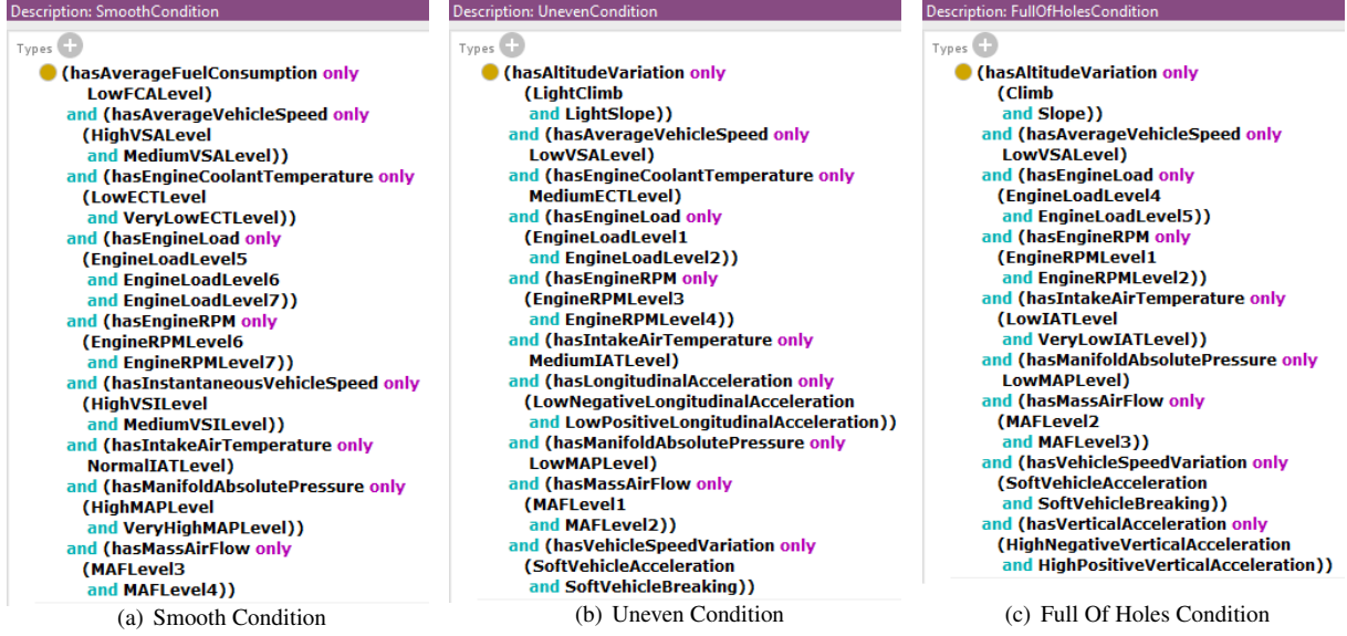
Fig. 8. Example of the model generated by MAFALDA for road surface
