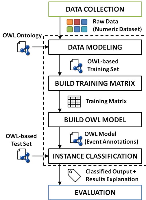
Fig. 1. Framework architecture
