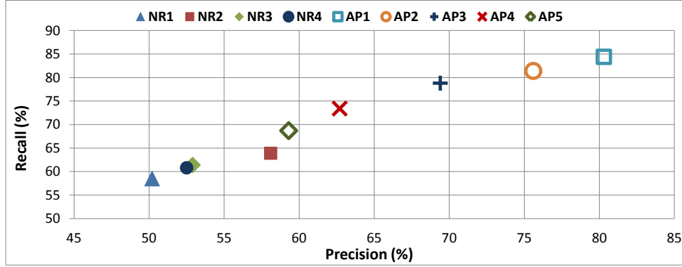
Fig. 6. Precision/recall plot
