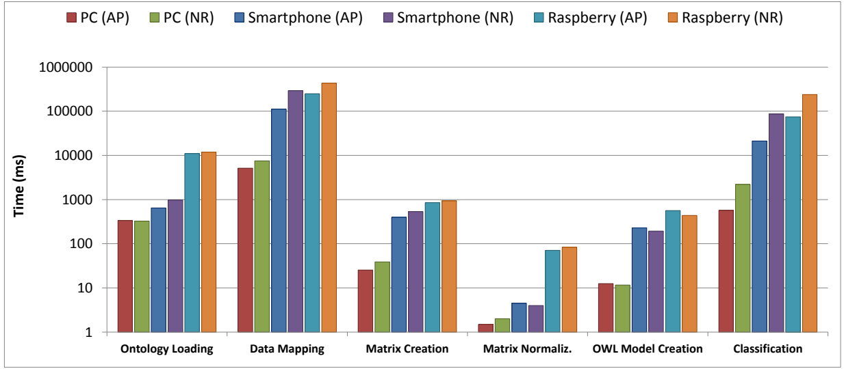
Fig. 7. Processing Time
