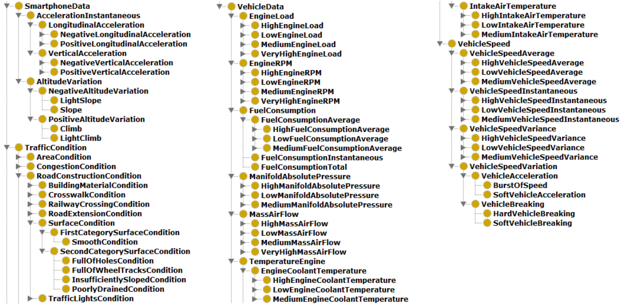
Fig. 2. Class hierarchy in the domain ontology for the case study
