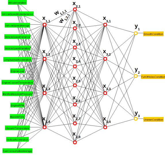
Fig. 10. Example of model for Multilayer Perceptron classifier
