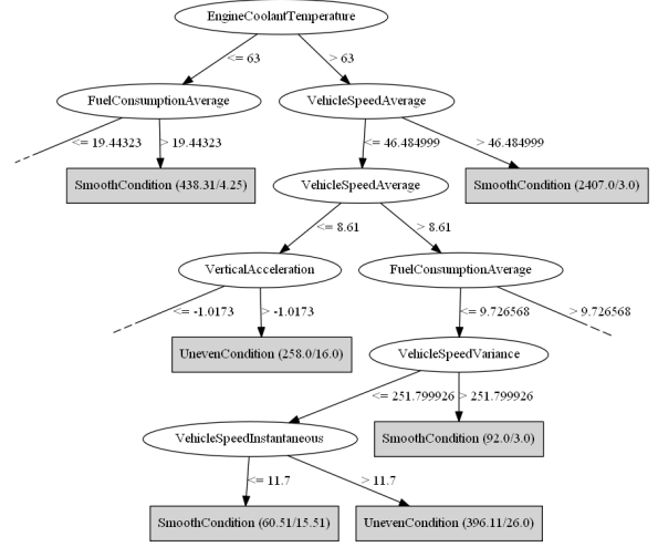
Fig. 8. Example of the model generated by MAFALDA for road surface
