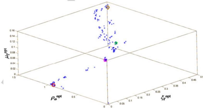
Figure 10. Space of design vector components by assuming also the mass ratio as design variable (case b).
