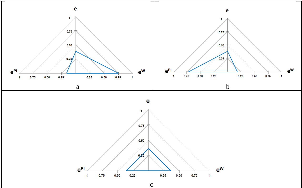
Figure 10. Graphical representation of the proposed ISN classification: (a) waste absorbing ISN; (b) primary input saving ISN; (c) balanced ISN. The same value of technical exchange efficiency can be obtained by ISNs with different e^W and e^{PI} .
