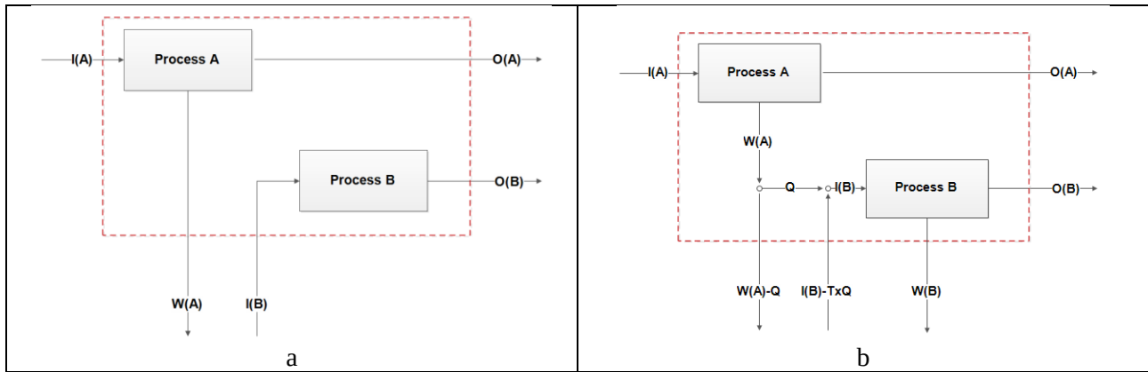
Figure 4. Industrial system composed by two production processes, when IS does not occur (a) and when IS occurs (b).
