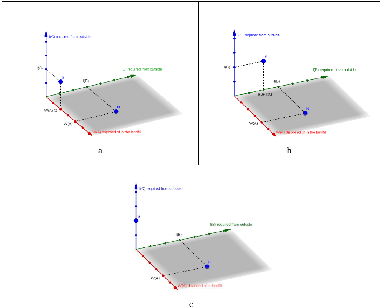
Figure 6. Effect of IS (when impure substitution occurs) on the efficient production frontier, in case: Q = \frac{I(B)}{T} < W(A) (a), Q = W(A) < \frac{I(B)}{T} (b), Q = W(A) = \frac{I(B)}{T} (c).
