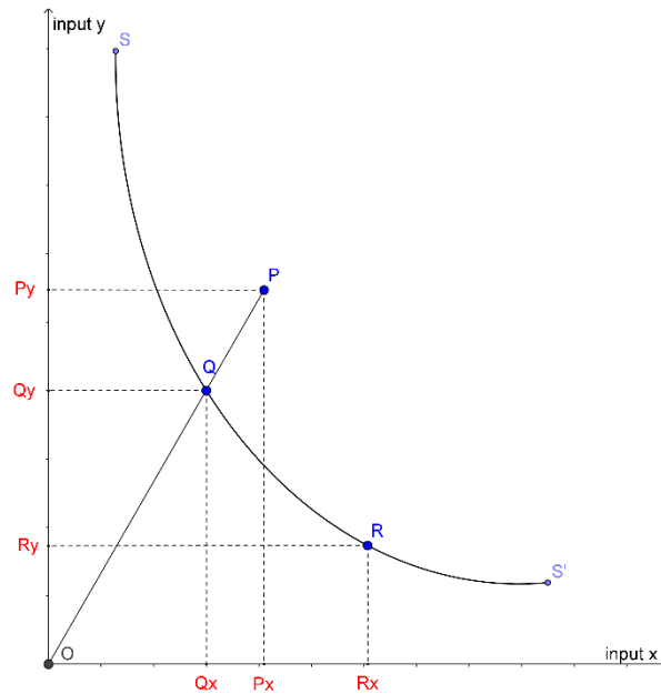
Figure 2. Graphical representation of the framework to evaluate technical production efficiency.
