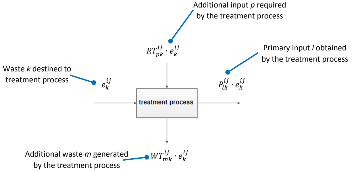
Figure 9. Graphical representation of the k -th waste treatment process in the ISN model.
