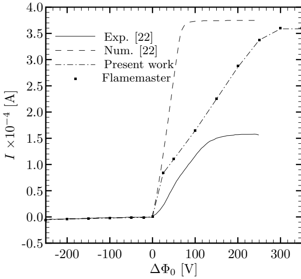
Figure S2.2: Electric intensity I as a function of the applied potential \Delta\Phi_0 . The three curves represent the experiments and numerical results of Speelman et al. [22], along with the present study. Symbols represent the solution obtained with Flamemaster.
