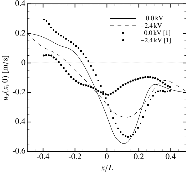
Figure 13: Comparison between numerical simulations (lines) and experimental measurements by Park et al. [1] (symbols) of the axial velocity profiles along the axis of the burner for Z_{st} = 0.07 .
