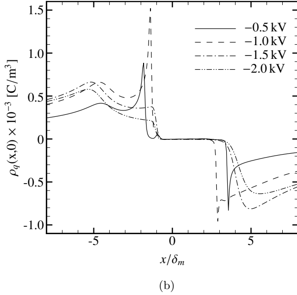
Figure 3: Dimensional charge density profiles along the axis of the burner for (a) Z_{st} = 0.07 and (b) Z_{st} = 0.50 .
