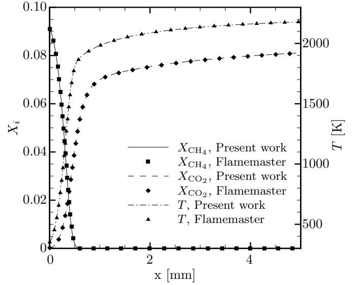
Figure S2.1: Spatial distributions of temperature and molar fractions of \text{CH}_4 and \text{CO}_2 through the flame. Symbols represent the solution obtained with Flamemaster, while lines correspond to results obtained with the present computational framework.
