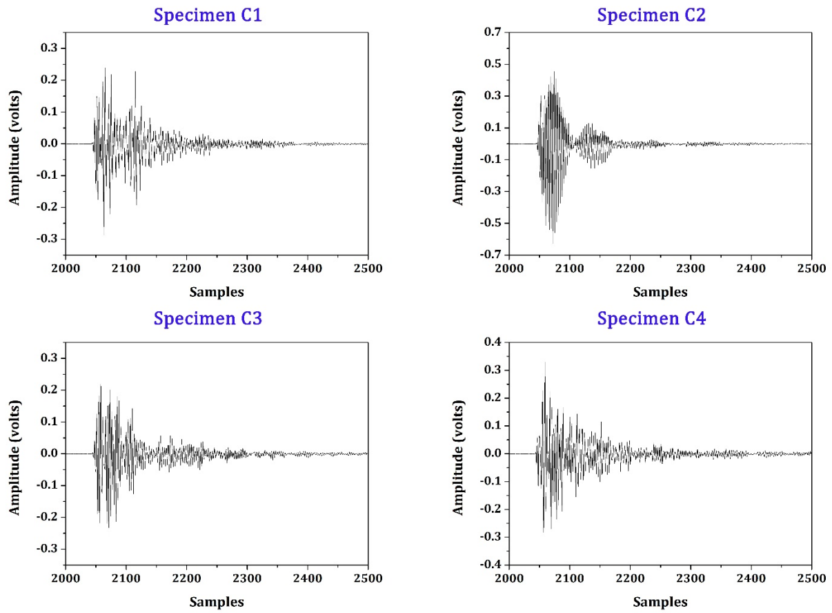
Figure 3. Waveform of the Received AE signals in different Specimens
