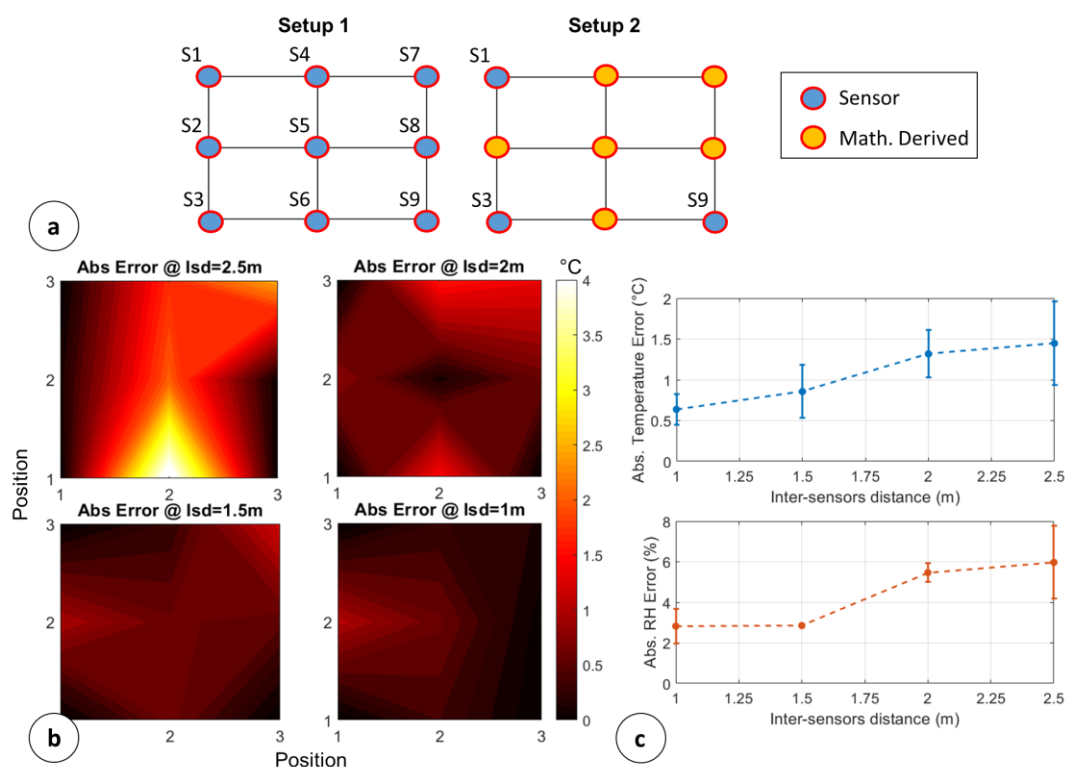
Figure 8. Absolute errors considering mathematically derived values: (a) ground truth setup (Setup1) vs. mathematically derived setup (b) absolute temperature errors with variable Isd (c) average and standard deviations of temperature and RH errors vs Isd.
