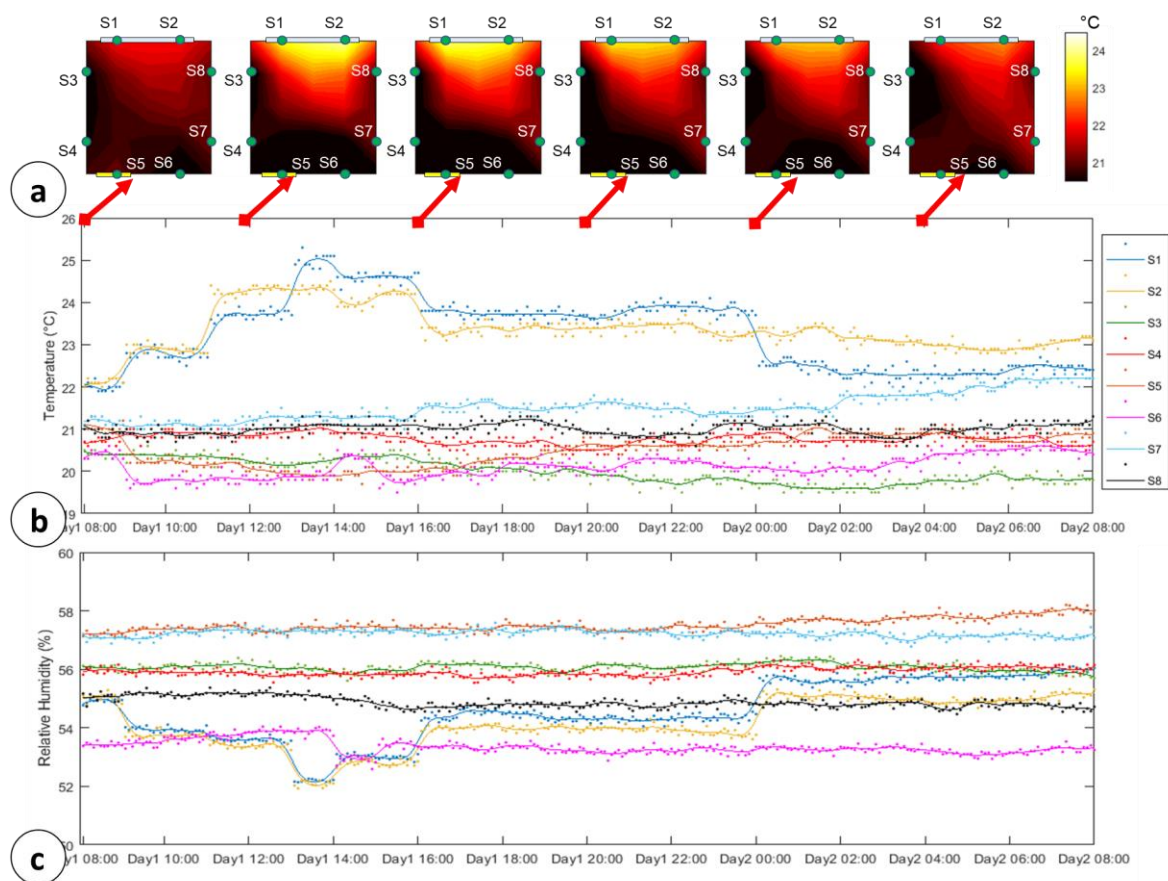
Figure 11. Sensors readings: (a) Testing room heat-map evolution during 24 h with step: 2 h (b) 24 h Temperature readings by n = 8 sensors (dots) and OLS estimations (solid line) (c) 24 h Humidity readings by n = 8 sensors (dots) and OLS estimations (solid line).
