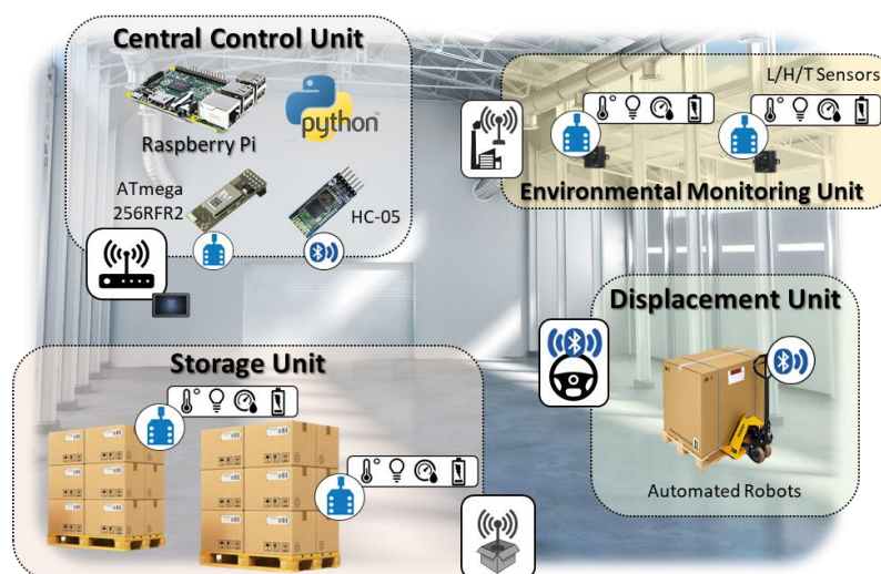
Figure 1. Top-level representation of the overall implemented architecture.
