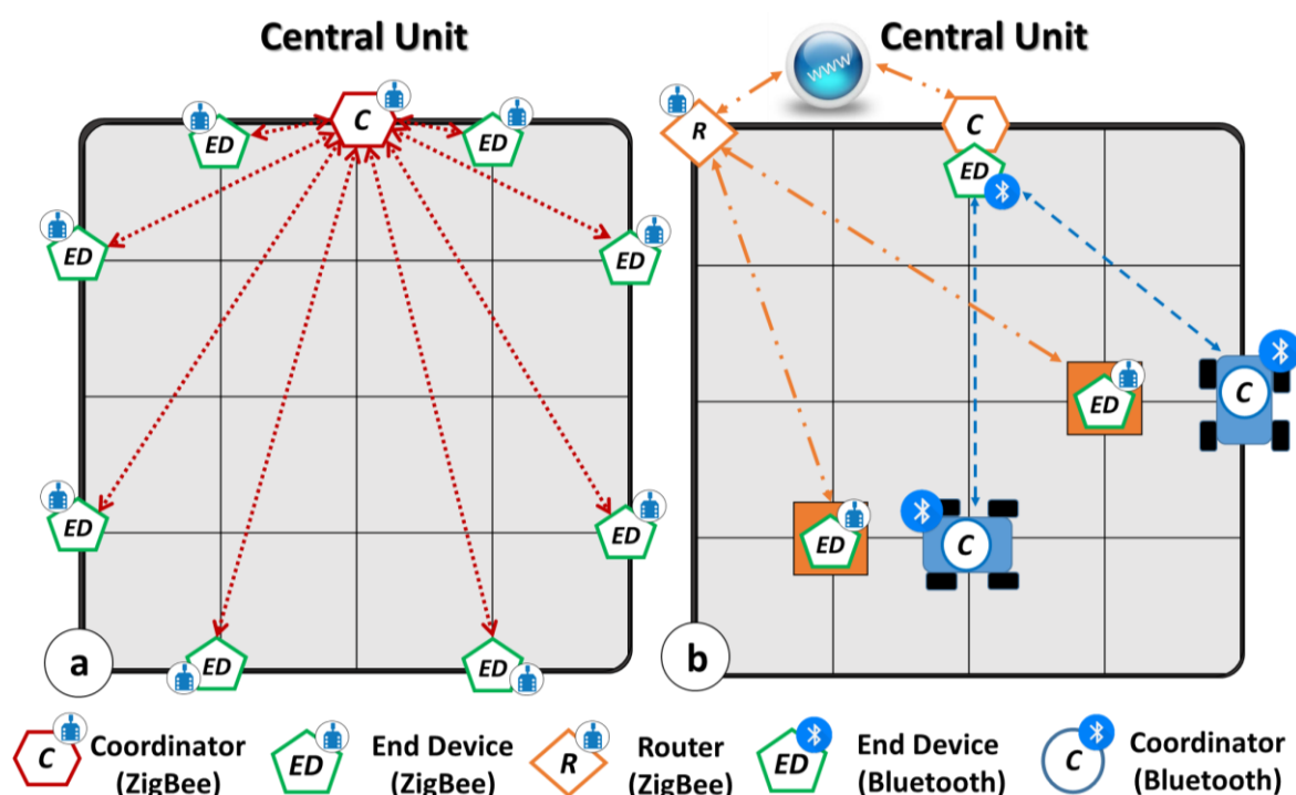
Figure 3. Communication Protocols: (a) Multipoint ZigBee Network for Environmental Control Unit (b) Router-based ZigBee Network for pallets monitoring and Bluetooth point-to-point Displacement Unit management.
