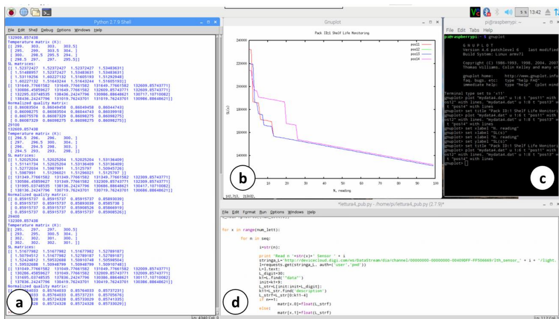
Figure 10. Screenshot of RPi-based Central Control Unit display: (a) Numeric monitoring of SL, C, T, etc. (b) Chart of SL monitoring of the selected positions for a specific pallet (c) Chart settings panel (d) HTTP-request panel for cloud reading.
