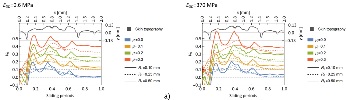
Figure X. Evolution of the cumulative global coefficient of friction along the sliding path as the indenter (of radius R_1 , R_2 and R_3 ) slides over the skin surface (one sliding period). The geometry of the skin surface is layered over this plot to relate evolution of global friction and geometric features of skin micro-relief. a) High relative humidity environment (Young's modulus of stratum corneum E_{SC} = 0.6 MPa); b) Low relative humidity environment ( E_{SC} = 370 MPa). Adapted from [250].
