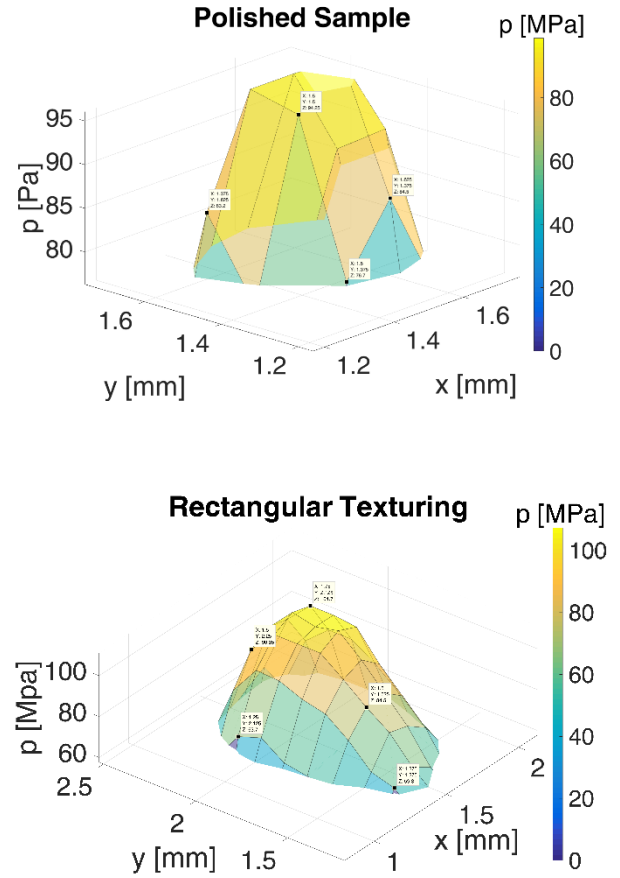
Figure 5: Contact pressure images (FPD-8010E)
