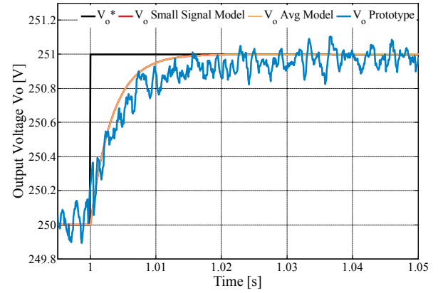
Fig. 13. DAB converters: response of the system in case of a reference voltage step \Delta V_o^* = 1V ( T_{\text{settling}} = 10\text{ms} ).
