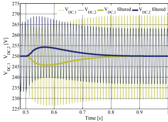
Fig. 17. CHB voltage balancing control: DC-link voltages in case of a power step for the two H-Bridges (simulation results).
