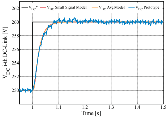
Fig. 12. CHB converter: response of the system in case of a reference voltage step \Delta V_{DC}^* = 10V ( T_{\text{settling}} = 100\text{ms} ).
