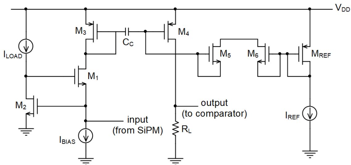
Fig. 14. The regulated common gate preamplifier of the ASIC TOFPET2.
