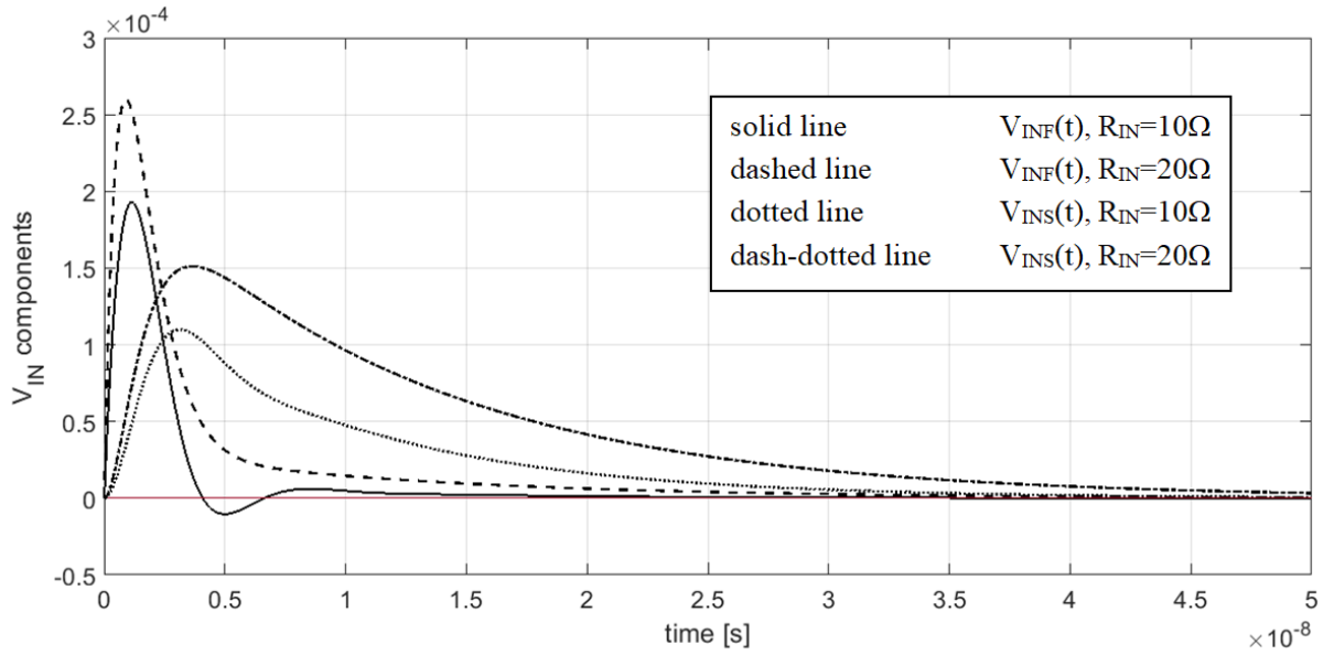
Fig. 5. Simulation of the fast and slow components of the signal V_{IN}(t) for two different values of R_{IN} , in presence of a parasitic interconnection inductance L=10\text{nH} .
