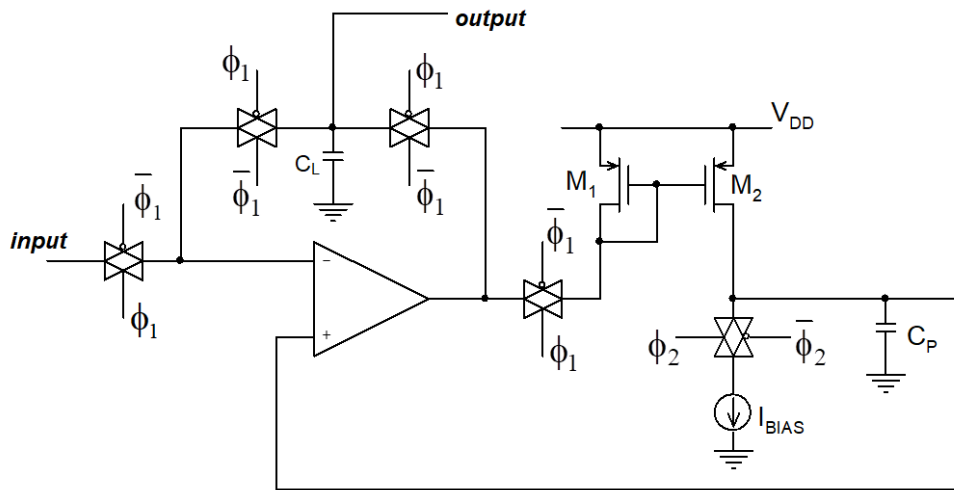
Fig. 19. Peak detection circuit.
