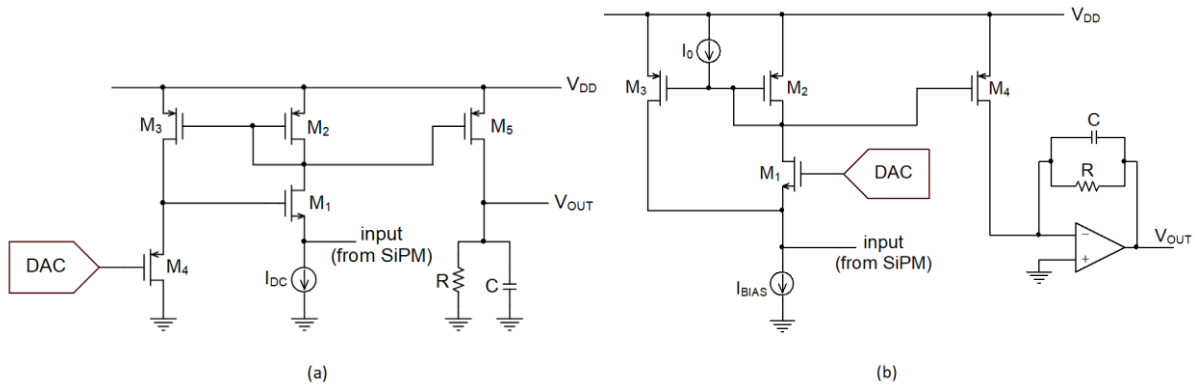
Fig. 18. Front-end and slow path of the analog channels of the ASICs Klaus (a) and BASIC (b).
