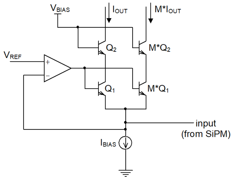
Fig. 16. Two signal paths formed directly at the input of the preamplifier by means of matched HBTs arranged in a regulated common base configuration.
