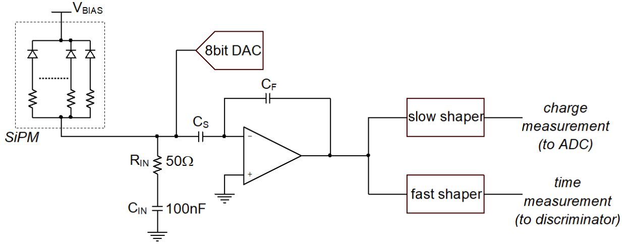
Fig. 8. Structure of the analog channel of the ASIC SPIROC.
