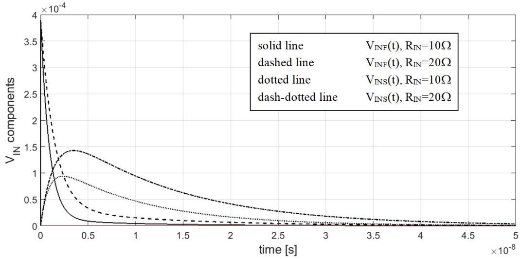
Fig. 4. Simulation of the fast and slow components of the signal V_{IN}(t) for two different values of R_{IN} .
