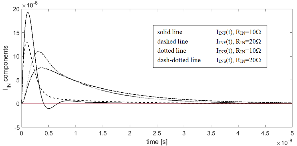
Fig. 6. Simulation of the fast and slow components of the current I_{IN}(t) for two different values of R_{IN} , in presence of a parasitic interconnection inductance L=10\text{nH} .
