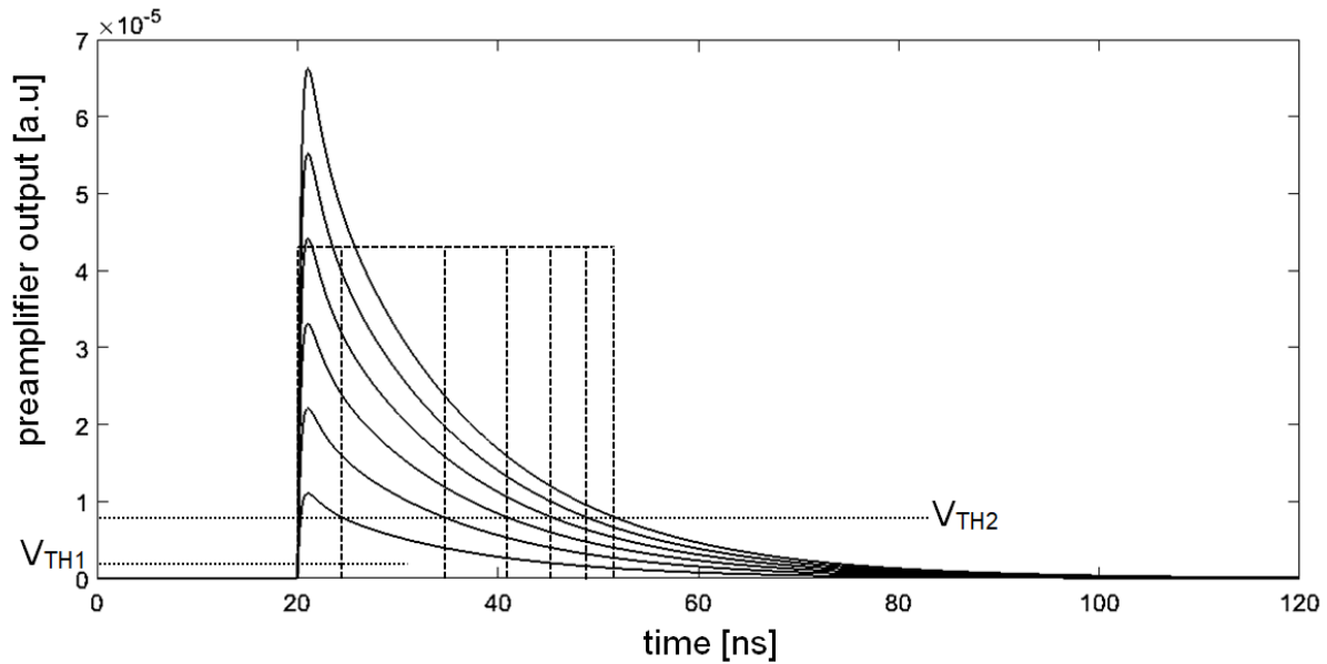
Fig. 22. Time over Threshold (ToT) technique for energy measurements.
