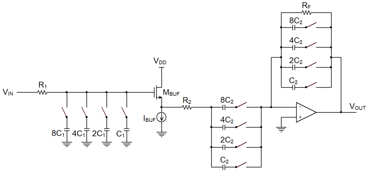
Fig. 17. Configuration of the CRRC 2 slow shaper used to integrate the output signal of the SPIROC preamplifier.
