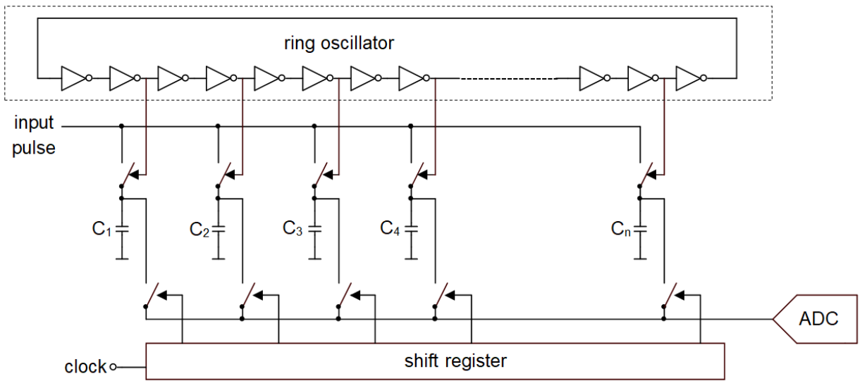
Fig. 26. An example of fast sampler: Domino structure.
