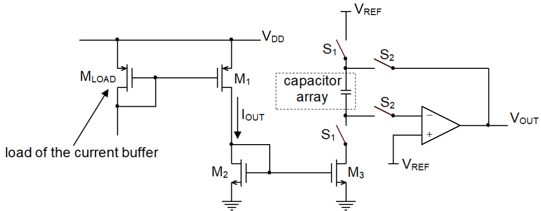
Fig. 20. Slow path of the ASIC TOFPET2.
