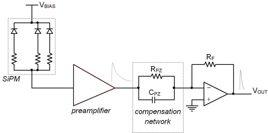
Fig. 25. The DLED technique, based on the compensation of the SiPM tail by means of pole-zero cancellation.
