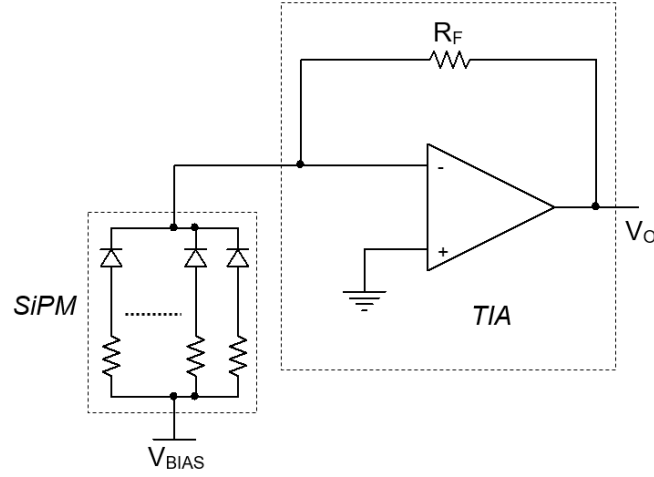
Fig. 2. Transimpedance amplifier (TIA) coupled to a SiPM.
