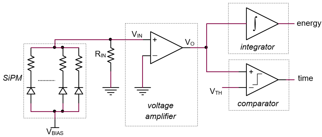
Fig. 7. SiPM readout with voltage mode approach.
