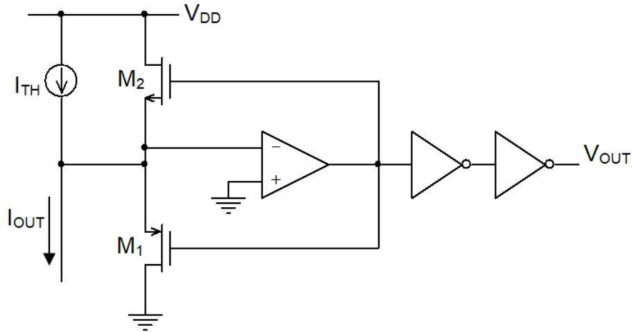
Fig. 24. Structure of a current discriminator.
