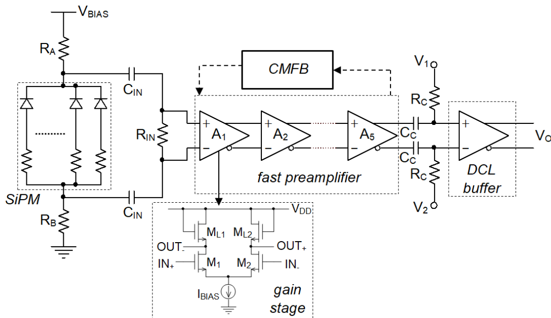
Fig. 9. Fast path of the ASIC PETA.
