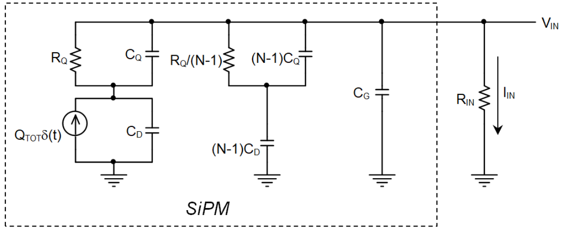
Fig. 3. SiPM model coupled to a generic preamplifier with input impedance R_{IN} .
