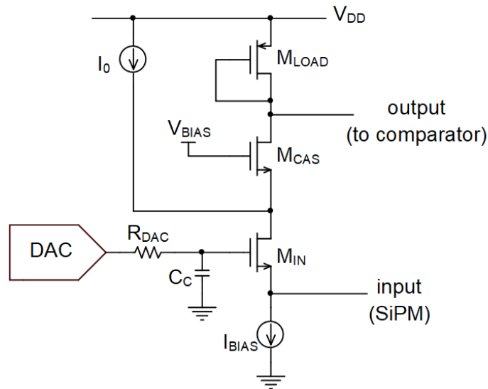
Fig. 12. Front-end of the ASIC STiC (only one branch of the differential current mode preamplifier).
