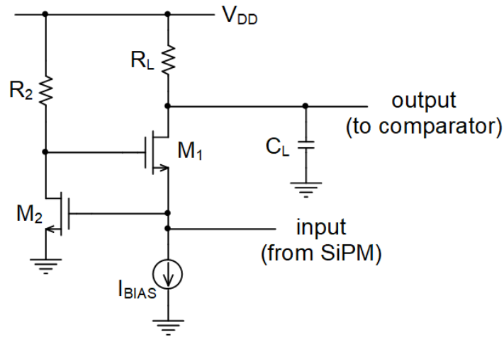
Fig. 13. Regulated common gate as a front-end for SiPM.
