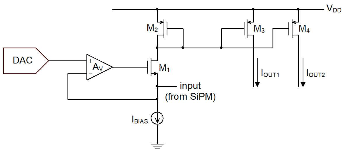
Fig. 15. Regulated common gate front-end with gain boosting realized by means of a differential amplifier.
