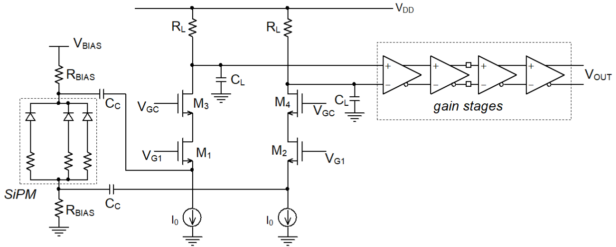
Fig. 11. Analog channel of the ASIC NINO.
