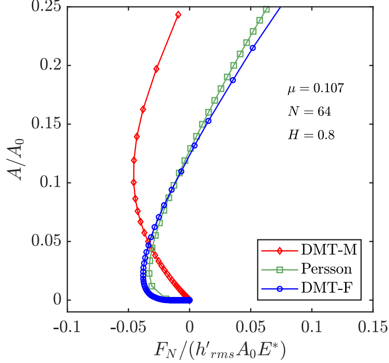
FIG. 7: The relative contact area A/A_0 as a function of the dimensionless applied load F_N/(E^* A_0 h'_{\text{rms}}) . Calculations are performed for \Delta\gamma = 0.2 J/m 2 , E^* = 1.33 \times 10^3 GPa and on a surface with N = 64 , H = 0.8 and h_{\text{rms}} = 0.52 nm, resulting in a Tabor parameter \mu = 0.107 . Persson's predictions are also plotted for comparison.
