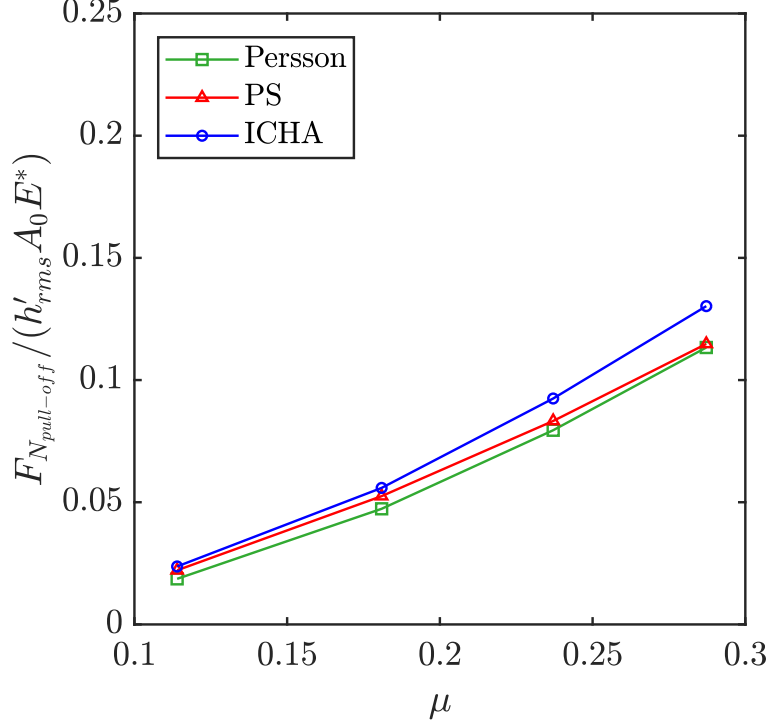
FIG. 2: The dimensionless pull-off force F_{N_{pull-off}}/(E^* A_0 h'_{rms}) as a function of the Tabor parameter \mu . Results are obtained on a self-affine surface with H = 0.8 , q_L = 2.5 \times 10^5 \text{ m}^{-1} , and q_0 = 4q_L . The PSD was truncated at q_1 = 64q_L , resulting in a root mean square roughness h_{rms} = 0.52 \text{ nm} and root mean square slope h'_{rms} = 0.00115 .
