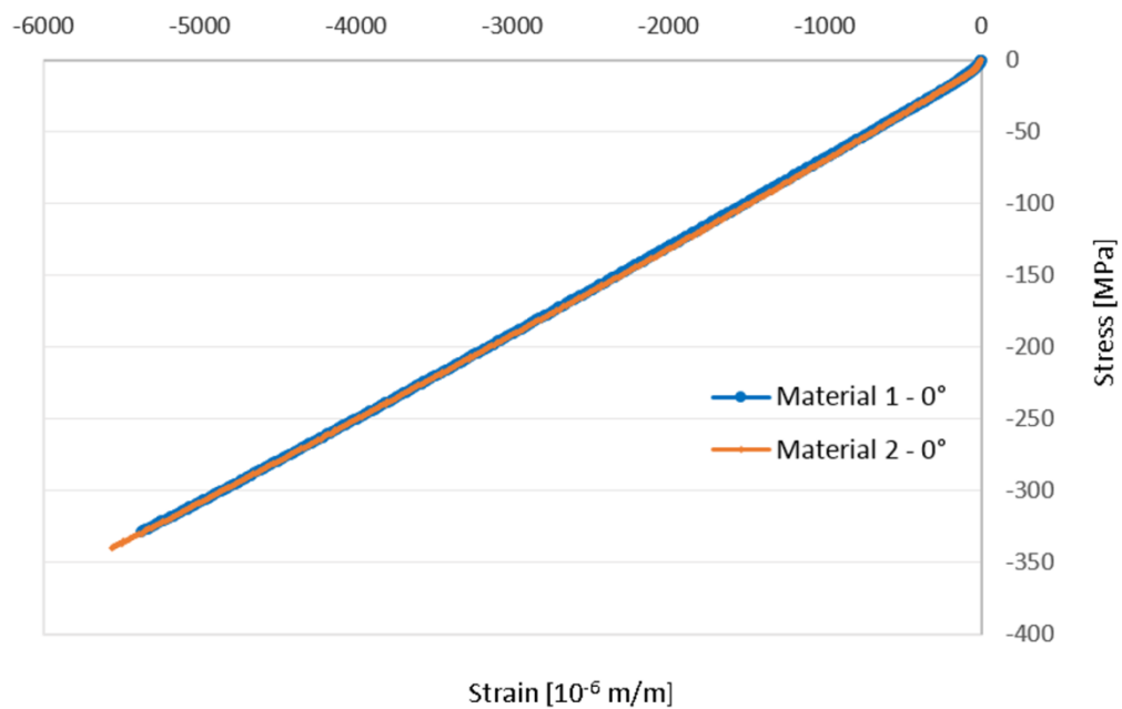
Figure 8. Compression Test 0°: Graphical Comparison
