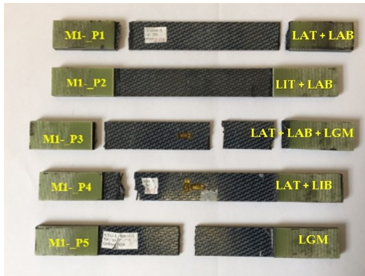
Figure 6. Tensile Test: Carbon/PEEK failure modes of specimens
