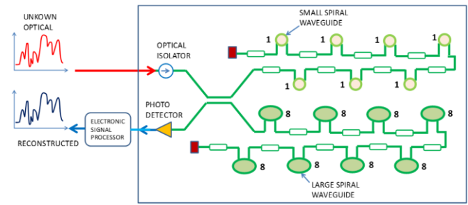
Fig. 1. On-chip layout of a digital Fourier transform spectrometer using a thermo-optical Michelson grating interferometer. Each red square represents an optical absorber. In the picture the numbers “8” and “1” indicate that the spiral lengths are in the ratio 8:1
