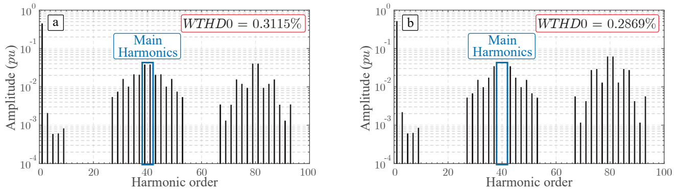
Fig. 6: Spectrum analysis for multilevel CHB with a clamped power cell with \phi = 60^\circ applying a) conventional PS-PWM b) proposed variable-angle PS-PWM.
